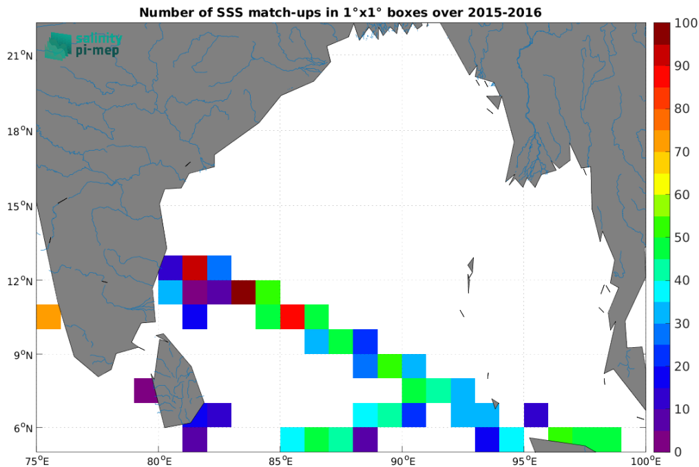
Figure 5: Number of SSS match-ups between TSG (LEGOS-DM) SSS and the SMAP SSS L2 v5.3 - 40 km (RSS) SSS product for the Ganga and Brahmaputra river plumes Pi-MEP region over 1^\circ \times 1^\circ boxes and for the full satellite product period.
