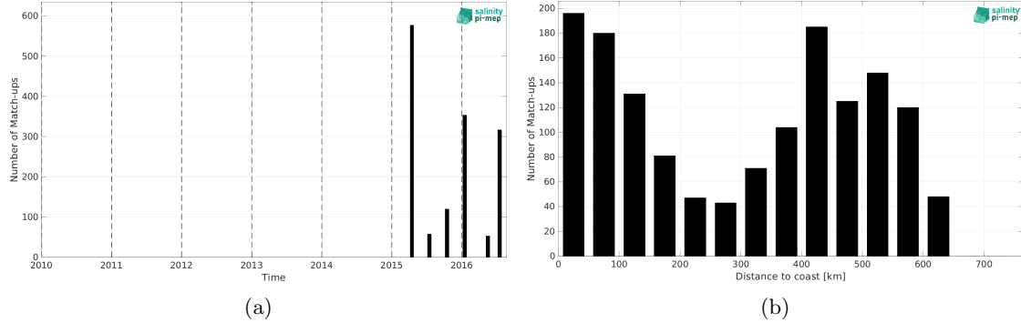
Figure 2: Number of match-ups between TSG (LEGOS-DM) and SMAP SSS L2 v5.3 - 40 km (RSS) SSS as a function of time (a) and as function of the distance to coast (b) over the Ganga and Brahmaputra river plumes Pi-MEP region and for the full satellite product period.
