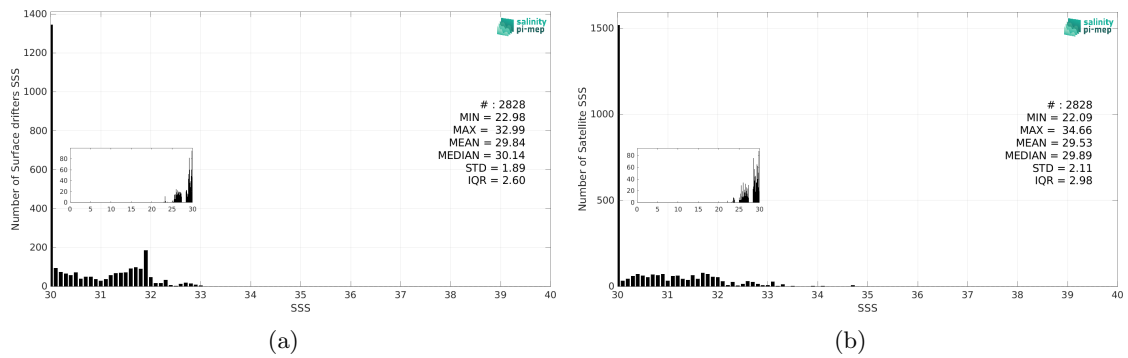
Figure 3: Histograms of SSS from Surface drifters (a) and SMAP SSS L2 v5.3 - 40 km (RSS) (b) considering all match-up pairs per bins of 0.1 over the Ganga and Brahmaputra river plumes Pi-MEP region and for the full satellite product period.
