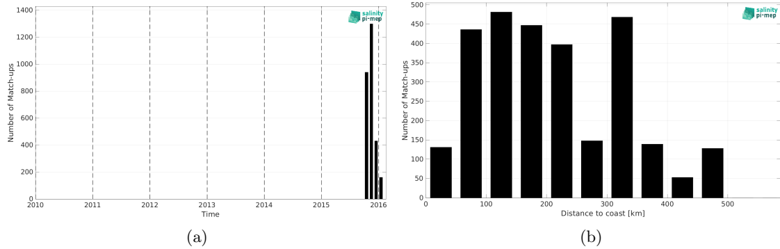
Figure 2: Number of match-ups between Surface drifters and SMAP SSS L2 v5.3 - 40 km (RSS) SSS as a function of time (a) and as function of the distance to coast (b) over the Ganga and Brahmaputra river plumes Pi-MEP region and for the full satellite product period.
