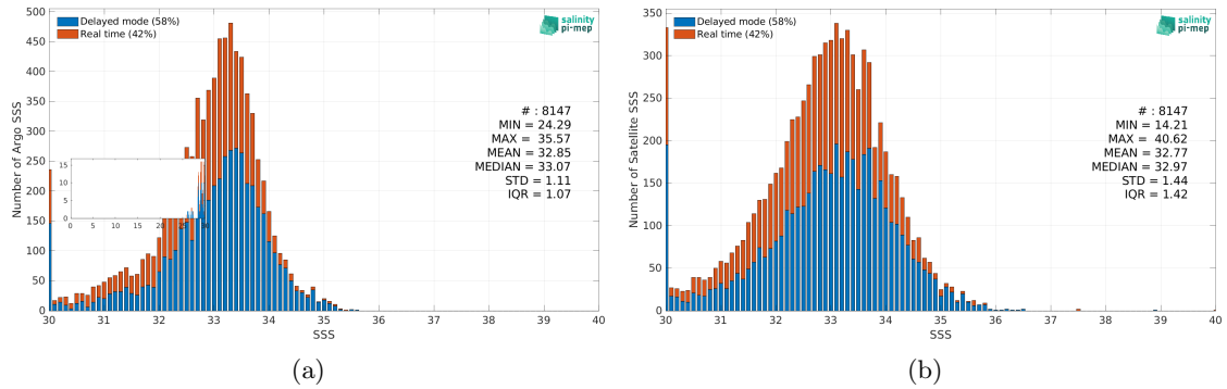
Figure 2: Histograms of SSS from Argo (a) and SMAP SSS L2 v5 - 40 km (RSS) (b) considering all match-up pairs per bins of 0.1 over the Ganga and Brahmaputra river plumes Pi-MEP region and for the full satellite product period.
