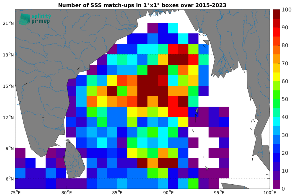
Figure 4: Number of SSS match-ups between Argo SSS and the SMAP SSS L2 v5 - 40 km (RSS) SSS product for the Ganga and Brahmaputra river plumes Pi-MEP region over 1^\circ \times 1^\circ boxes and for the full satellite product period.
