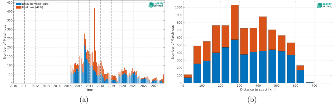
Figure 1: Number of match-ups between Argo and SMAP SSS L2 v5 - 40 km (RSS) SSS as a function of time (a) and as function of the distance to coast (b) over the Ganga and Brahmaputra river plumes Pi-MEP region and for the full satellite product period.
