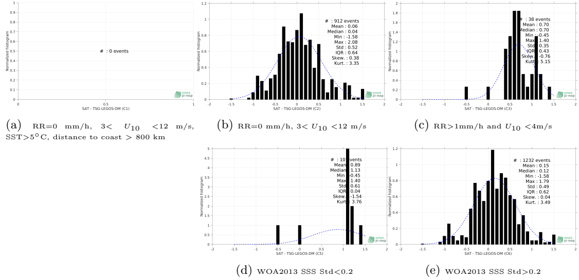
Figure 13: Normalized histogram of \Delta SSS (SMAP-L2-RSS-V4 - TSG-LEGOS-DM) for 5 different subdatasets corresponding to: RR=0 mm/h, 3 < U_{10} < 12 m/s, SST>5°C, distance to coast > 800 km (a), RR=0 mm/h, 3 < U_{10} < 12 m/s (b), RR>1mm/h and U_{10} < 4 m/s (c), WOA2013 SSS Std<0.2 (d), WOA2013 SSS Std>0.2 (e).
