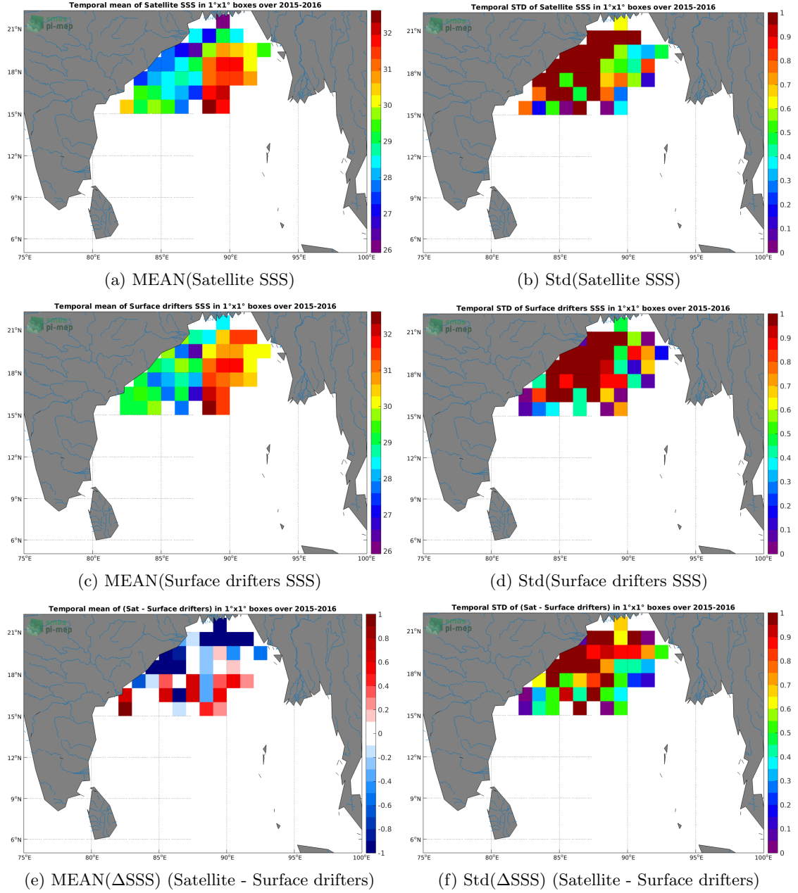
Figure 5: Temporal mean (left) and Std (right) of SSS from SMAP SSS L2 v4 (RSS) (top), Surface drifters (middle), and of \Delta SSS (Satellite - Surface drifters). Only match-up pairs are used to generate these maps.
