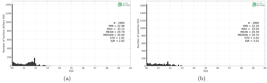
Figure 2: Histograms of SSS from Surface drifters (a) and SMAP SSS L2 v4 (RSS) (b) considering all match-up pairs per bins of 0.1 over the Ganga and Brahmaputra river plumes Pi-MEP region and for the full satellite product period.
