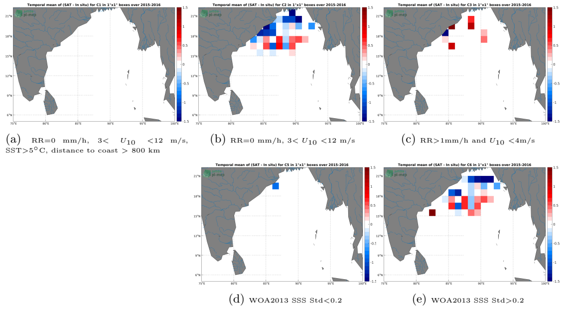
Figure 11: Temporal mean gridded over spatial boxes of size 1^\circ \times 1^\circ of \Delta SSS (SMAP SSS L2 v4 (RSS) - Surface drifters) for 5 different subdatasets corresponding to: RR=0 mm/h, 3 < U_{10} < 12 m/s, SST > 5^\circ\text{C} , distance to coast > 800 km (a), RR=0 mm/h, 3 < U_{10} < 12 m/s (b), RR > 1 mm/h and U_{10} < 4 m/s (c), WOA2013 SSS Std < 0.2 (d), WOA2013 SSS Std > 0.2 (e).
