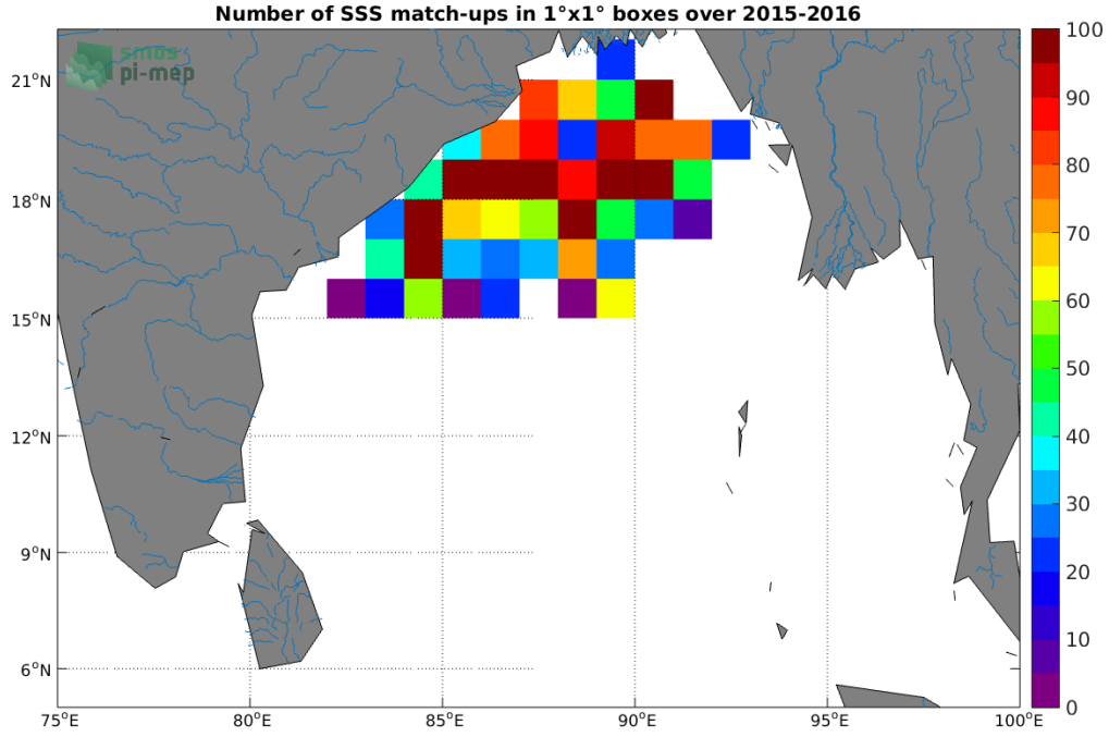
Figure 3: Number of SSS match-ups between Surface drifters SSS and the SMAP SSS L2 v4 (RSS) SSS product for the Ganga and Brahmaputra river plumes Pi-MEP region over 1^\circ \times 1^\circ boxes and for the full satellite product period.
