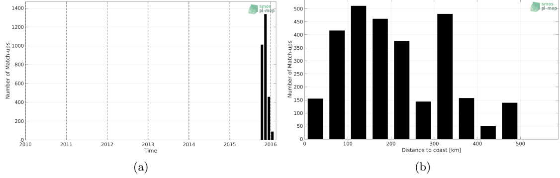
Figure 1: Number of match-ups between Surface drifters and SMAP SSS L2 v4 (RSS) SSS as a function of time (a) and as function of the distance to coast (b) over the Ganga and Brahmaputra river plumes Pi-MEP region and for the full satellite product period.
