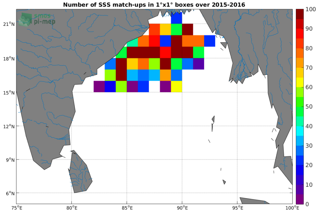
Figure 3: Number of SSS match-ups between Surface drifters SSS and the SMAP SSS L2 v4 (RSS) SSS product for the Ganga and Brahmaputra river plumes Pi-MEP region over 1°x1° boxes and for the full satellite product period.
