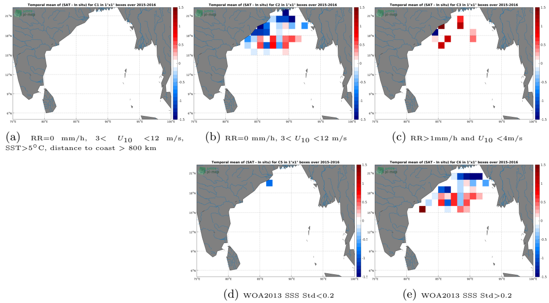
Figure 11: Temporal mean gridded over spatial boxes of size 1^\circ \times 1^\circ of \Delta SSS (SMAP SSS L2 v4 (RSS) - Surface drifters) for 5 different subdatasets corresponding to:RR=0 mm/h, 3 < U_{10} < 12 m/s, SST >5^\circ\text{C} , distance to coast > 800 km (a), RR=0 mm/h, 3 < U_{10} < 12 m/s (b), RR >1 mm/h and U_{10} < 4 m/s (c), WOA2013 SSS Std <0.2 (d), WOA2013 SSS Std >0.2 (e).
