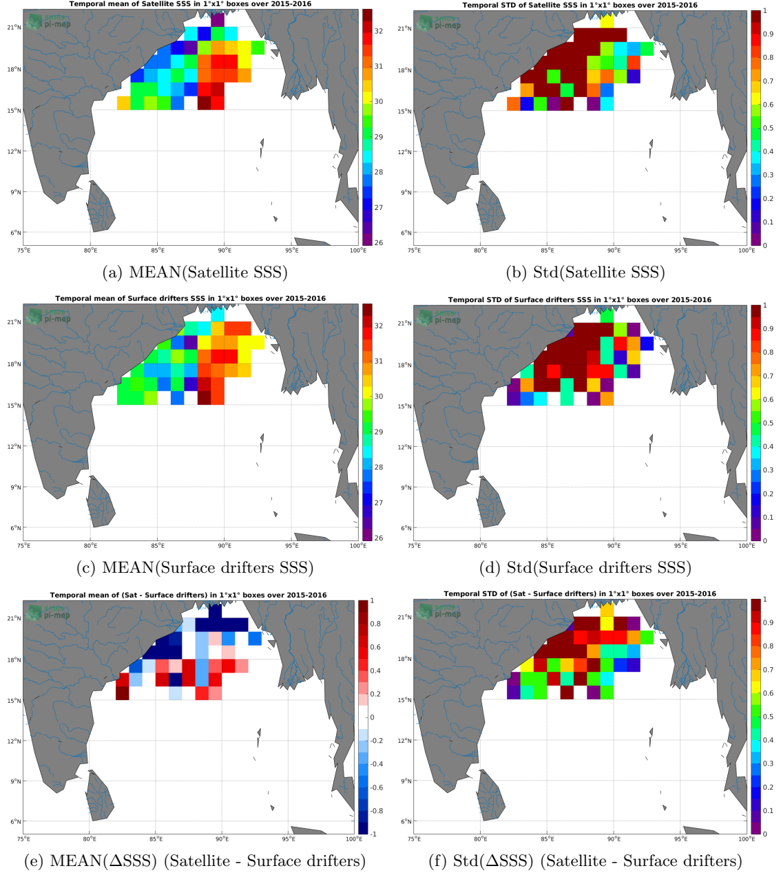
Figure 5: Temporal mean (left) and Std (right) of SSS from SMAP-L2-RSS-V4 (top), Surface drifters (middle), and of ΔSSS (Satellite - Surface drifters). Only match-up pairs are used to generate these maps.
