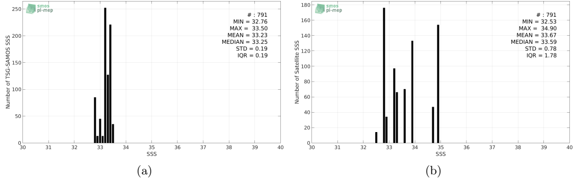
Figure 2: Histograms of SSS from TSG-SAMOS (a) and SMAP-L2-RSS-V3-70KM (b) considering all match-up pairs per bins of 0.1 over the Ganga and Brahmaputra river plumes Pi-MEP region and for the full satellite product period.
