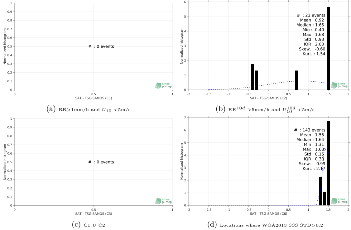
Figure 13: Normalized histogram of \Delta\text{SSS} (SMAP-L2-RSS-V3-70KM - TSG-SAMOS) for 6 different subdatasets corresponding to: RR > 1\text{mm/h} and U_{10} < 5\text{m/s} (a), RR^{10d} > 5\text{mm/h} and U_{10}^{10d} < 5\text{m/s} (b), C1 U C2 (c), Locations where WOA2013 SSS STD > 0.2 (d).
