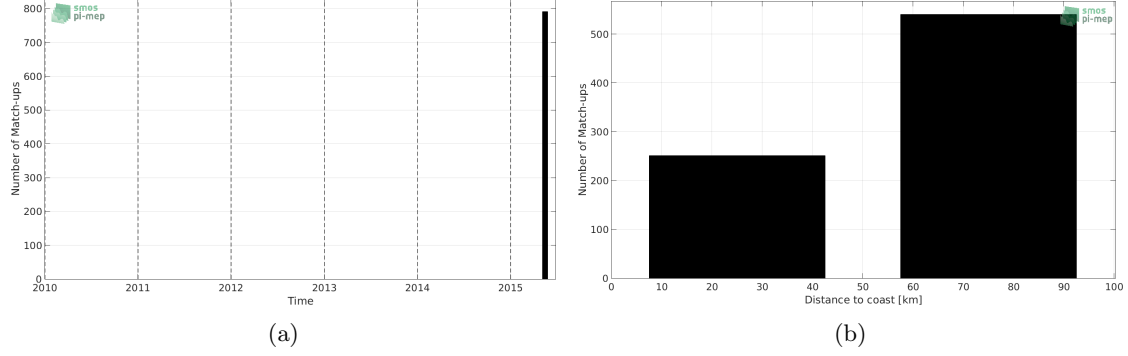
Figure 1: Number of match-ups between TSG-SAMOS and SMAP-L2-RSS-V3-70KM SSS as a function of time (a) and as function of the distance to coast (b) over the Ganga and Brahmaputra river plumes Pi-MEP region and for the full satellite product period.
