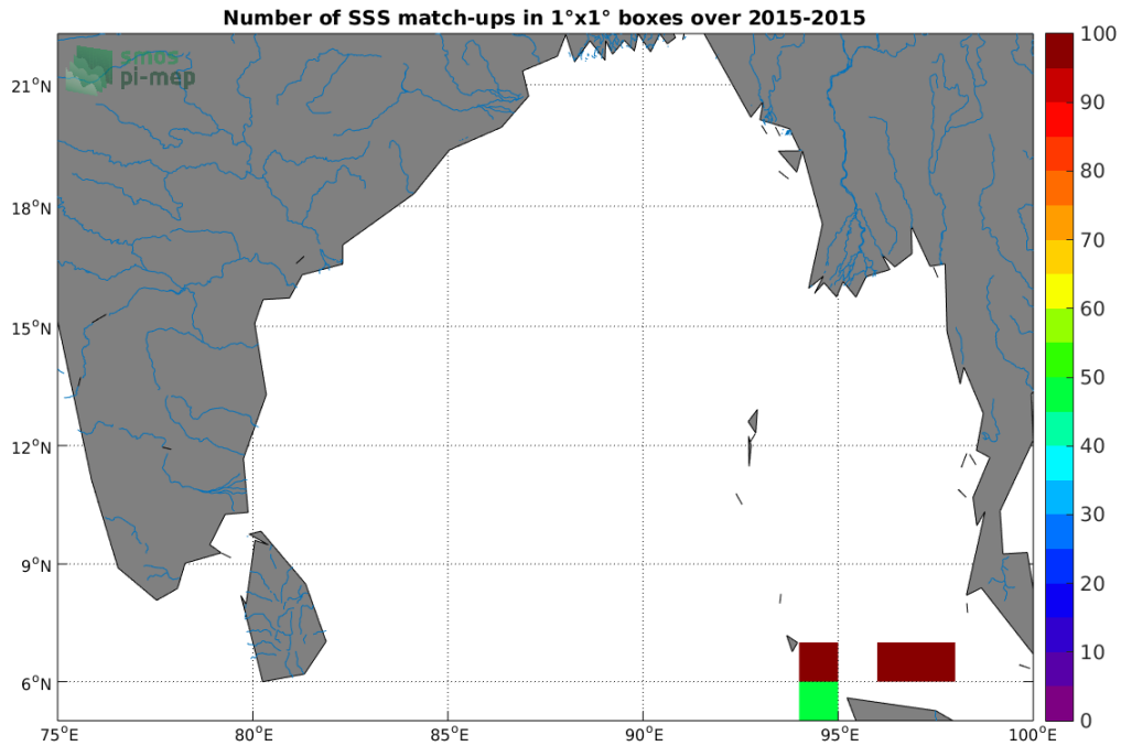
Figure 4: Number of SSS match-ups between TSG-SAMOS SSS and the SMAP-L2-RSS-V3-70KM SSS product for the Ganga and Brahmaputra river plumes Pi-MEP region over 1^\circ \times 1^\circ boxes and for the full satellite product period.
