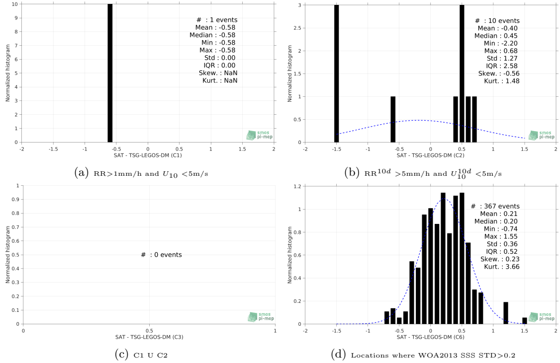
Figure 13: Normalized histogram of \Delta\text{SSS} (SMAP-L2-RSS-V3-70KM - TSG-LEGOS-DM) for 6 different subdatasets corresponding to: RR > 1mm/h and U_{10} < 5\text{m/s} (a), RR^{10d} > 5\text{mm/h} and U_{10}^{10d} < 5\text{m/s} (b), C1 U C2 (c), Locations where WOA2013 SSS STD > 0.2 (d).
