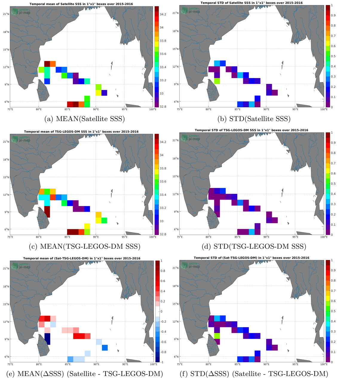
Figure 6: Temporal mean (left) and STD (right) of SSS from SMAP-L2-RSS-V3-70KM (top), TSG-LEGOS-DM (middle), and of \Delta SSS (Satellite - TSG-LEGOS-DM). Only match-up pairs are used to generate these maps.
