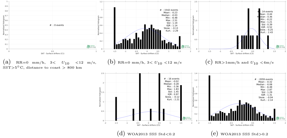
Figure 12: Normalized histogram of \Delta SSS (SMAP-L2-RSS-V3-70KM - Surface drifters) for 5 different subdatasets corresponding to: RR=0 mm/h, 3 < U_{10} < 12 m/s, SST > 5°C, distance to coast > 800 km (a), RR=0 mm/h, 3 < U_{10} < 12 m/s (b), RR > 1mm/h and U_{10} < 4 m/s (c), WOA2013 SSS Std < 0.2 (d), WOA2013 SSS Std > 0.2 (e).
