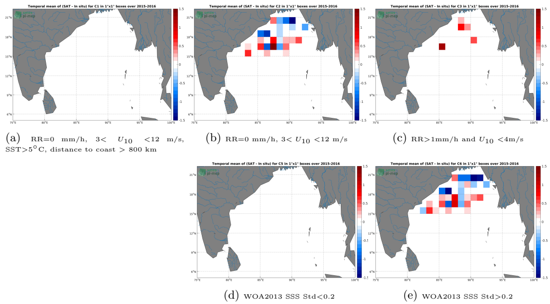
Figure 11: Temporal mean gridded over spatial boxes of size 1^\circ \times 1^\circ of \Delta SSS (SMAP-L2-RSS-V3-70KM - Surface drifters) for 5 different subdatasets corresponding to:RR=0 mm/h, 3 < U_{10} < 12 m/s, SST >5^\circ C, distance to coast > 800 km (a), RR=0 mm/h, 3 < U_{10} < 12 m/s (b), RR >1 mm/h and U_{10} < 4 m/s (c), WOA2013 SSS Std <0.2 (d), WOA2013 SSS Std >0.2 (e).
