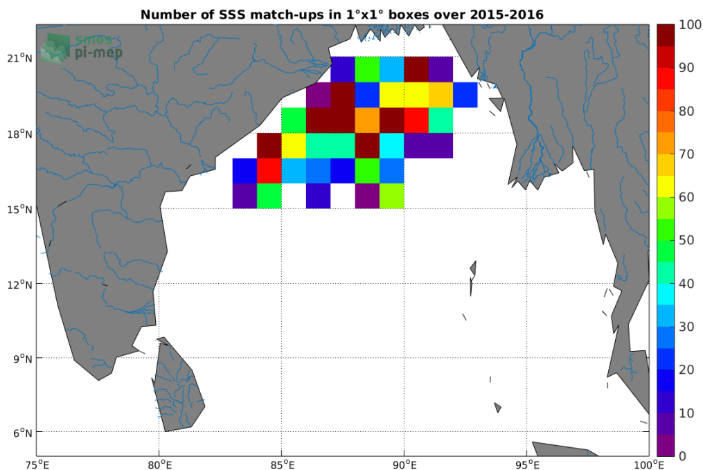
Figure 3: Number of SSS match-ups between Surface drifters SSS and the SMAP-L2-RSS-V3-70KM SSS product for the Ganga and Brahmaputra river plumes Pi-MEP region over 1^\circ \times 1^\circ boxes and for the full satellite product period.
