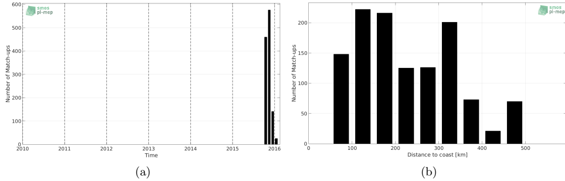
Figure 1: Number of match-ups between Surface drifters and SMAP-L2-RSS-V3-70KM SSS as a function of time (a) and as function of the distance to coast (b) over the Ganga and Brahmaputra river plumes Pi-MEP region and for the full satellite product period.
