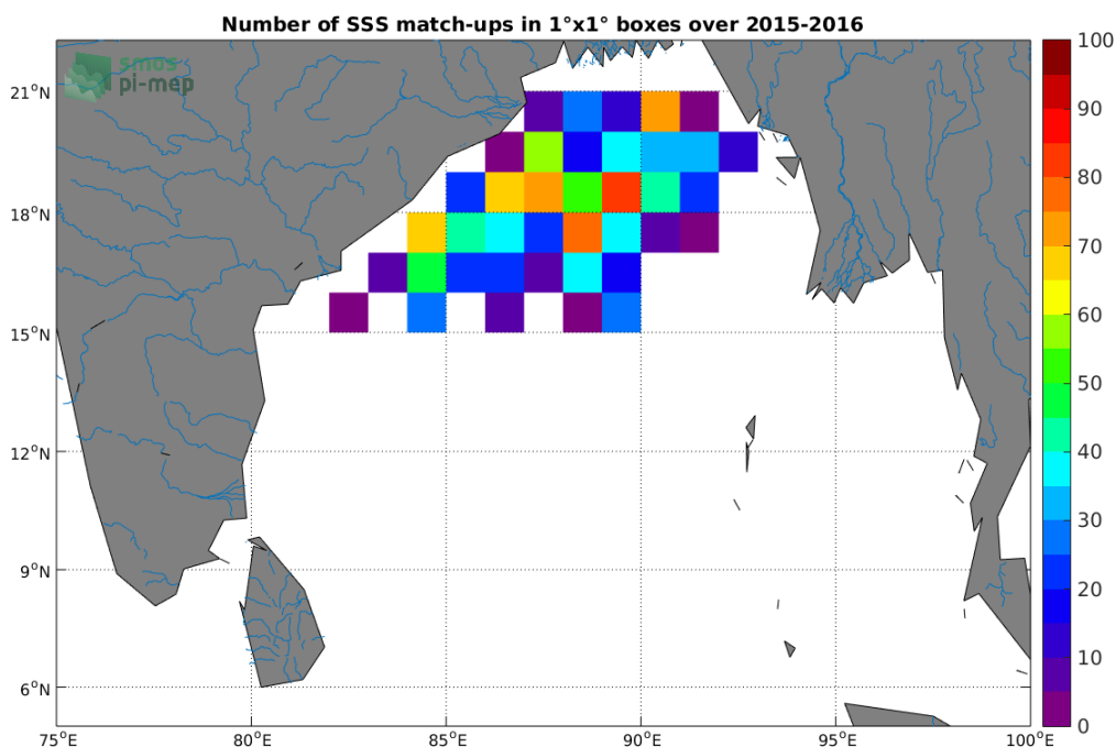
Figure 3: Number of SSS match-ups between Surface drifters SSS and the SMAP-L2-RSS-V3-70KM SSS product for the Ganga and Brahmaputra river plumes Pi-MEP region over 1°x1° boxes and for the full satellite product period.
