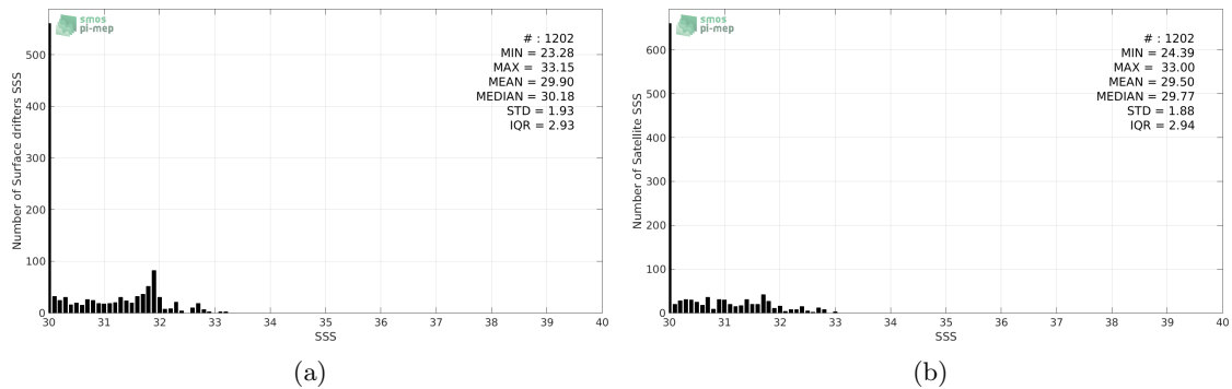
Figure 2: Histograms of SSS from Surface drifters (a) and SMAP-L2-RSS-V3-70KM (b) considering all match-up pairs per bins of 0.1 over the Ganga and Brahmaputra river plumes Pi-MEP region and for the full satellite product period.
