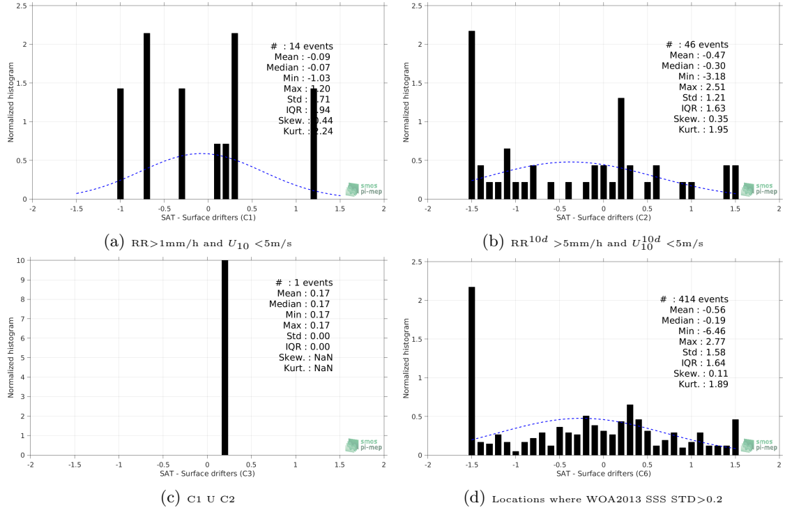
Figure 12: Normalized histogram of \Delta SSS (SMAP-L2-RSS-V3-70KM - Surface drifters) for 6 different subdatasets corresponding to: RR > 1\text{mm/h} and U_{10} < 5\text{m/s} (a), RR^{10d} > 5\text{mm/h} and U_{10}^{10d} < 5\text{m/s} (b), C1 U C2 (c), Locations where WOA2013 SSS STD > 0.2 (d).
