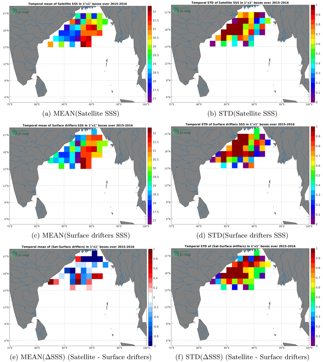
Figure 5: Temporal mean (left) and STD (right) of SSS from SMAP-L2-RSS-V3-70KM (top), Surface drifters (middle), and of \Delta SSS (Satellite - Surface drifters). Only match-up pairs are used to generate these maps.
