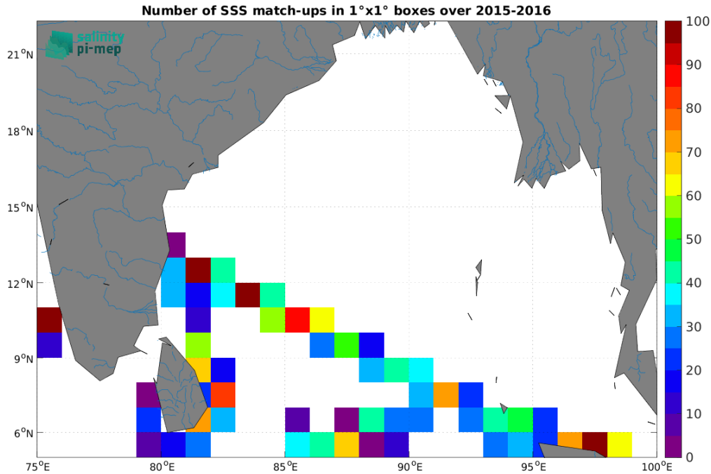
Figure 5: Number of SSS match-ups between TSG (LEGOS-DM) SSS and the SMAP SSS L2 v5.0 (JPL) SSS product for the Ganga and Brahmaputra river plumes Pi-MEP region over 1^{\circ} \times 1^{\circ} boxes and for the full satellite product period.
