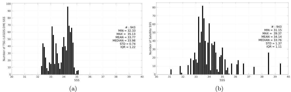
Figure 3: Histograms of SSS from TSG (LEGOS-DM) (a) and SMAP SSS L2 v5.0 (JPL) (b) considering all match-up pairs per bins of 0.1 over the Ganga and Brahmaputra river plumes Pi-MEP region and for the full satellite product period.
