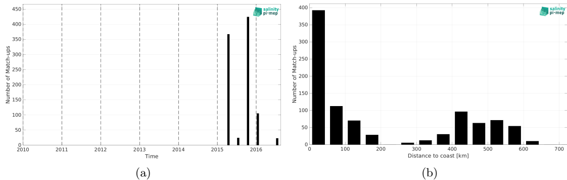
Figure 2: Number of match-ups between TSG (LEGOS-DM) and SMAP SSS L2 v5.0 (JPL) SSS as a function of time (a) and as function of the distance to coast (b) over the Ganga and Brahmaputra river plumes Pi-MEP region and for the full satellite product period.
