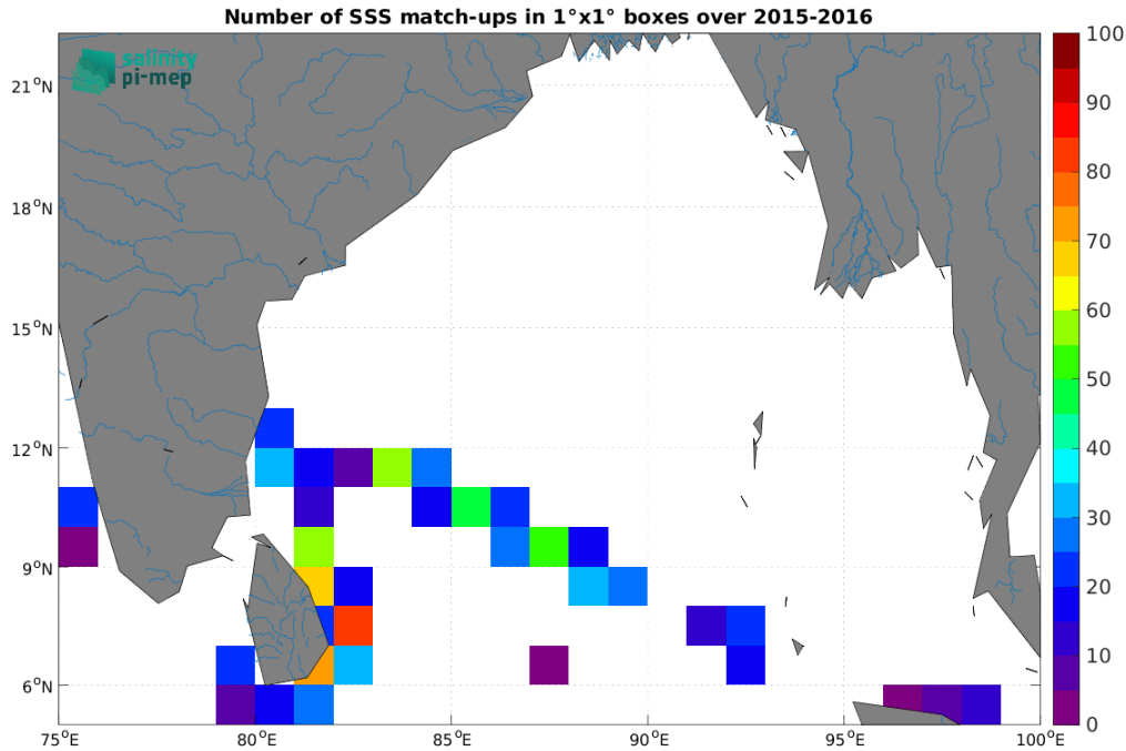
Figure 5: Number of SSS match-ups between TSG (LEGOS-DM) SSS and the SMAP SSS L2 v5.0 (JPL) SSS product for the Ganga and Brahmaputra river plumes Pi-MEP region over 1^\circ \times 1^\circ boxes and for the full satellite product period.
