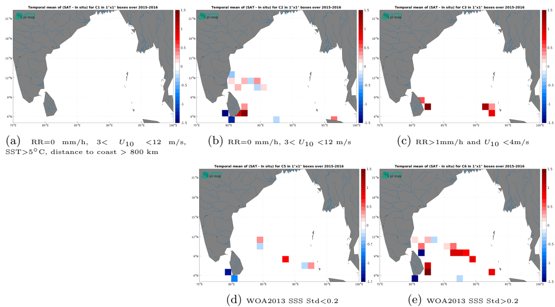
Figure 14: Temporal mean gridded over spatial boxes of size 1^\circ \times 1^\circ of \Delta SSS (SMAP SSS L2 v5.0 (JPL) - TSG (LEGOS-DM)) for 5 different subdatasets corresponding to:RR=0 mm/h, 3 < U_{10} < 12 m/s, SST>5°C, distance to coast > 800 km (a), RR=0 mm/h, 3 < U_{10} < 12 m/s (b), RR>1mm/h and U_{10} < 4 m/s (c), WOA2013 SSS Std<0.2 (d), WOA2013 SSS Std>0.2 (e).
