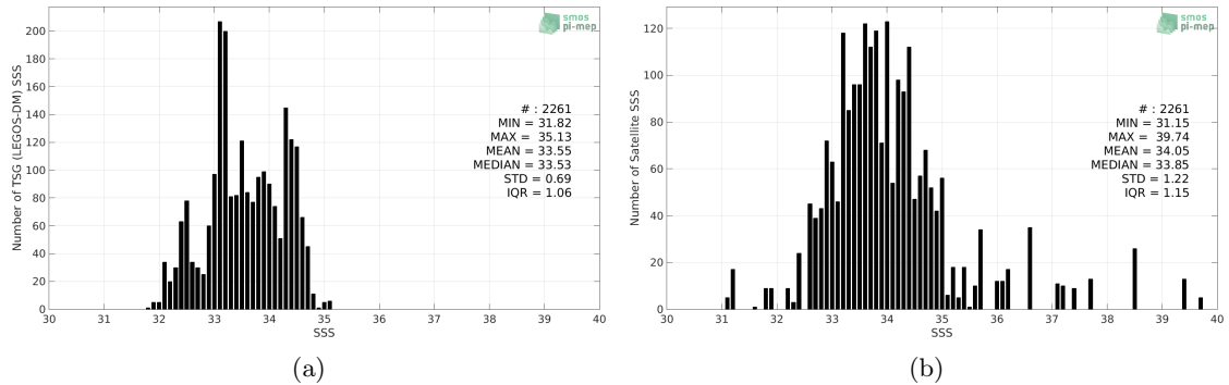
Figure 2: Histograms of SSS from TSG (LEGOS-DM) (a) and SMAP SSS L2 v5.0 (JPL) (b) considering all match-up pairs per bins of 0.1 over the Ganga and Brahmaputra river plumes Pi-MEP region and for the full satellite product period.
