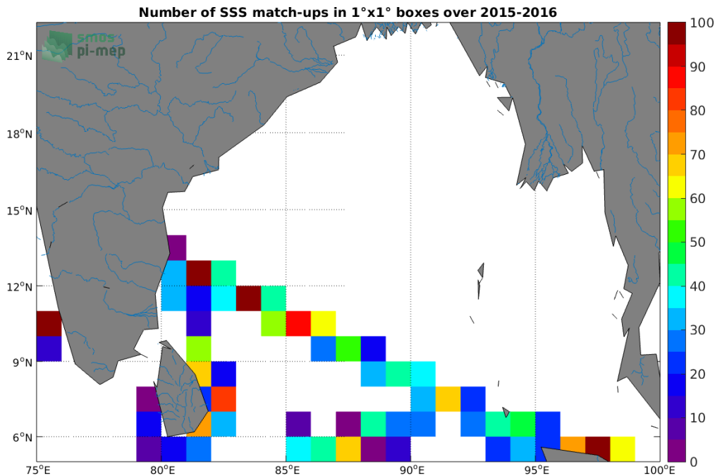
Figure 4: Number of SSS match-ups between TSG (LEGOS-DM) SSS and the SMAP SSS L2 v5.0 (JPL) SSS product for the Ganga and Brahmaputra river plumes Pi-MEP region over 1°x1° boxes and for the full satellite product period.
