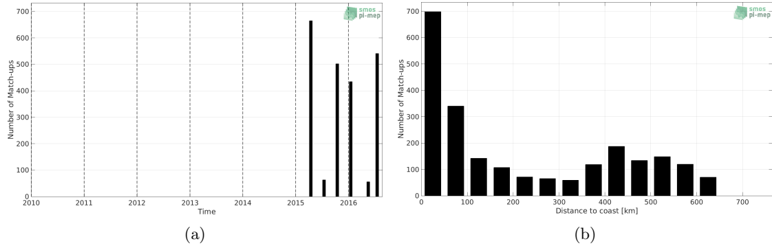
Figure 1: Number of match-ups between TSG (LEGOS-DM) and SMAP SSS L2 v5.0 (JPL) SSS as a function of time (a) and as function of the distance to coast (b) over the Ganga and Brahmaputra river plumes Pi-MEP region and for the full satellite product period.
