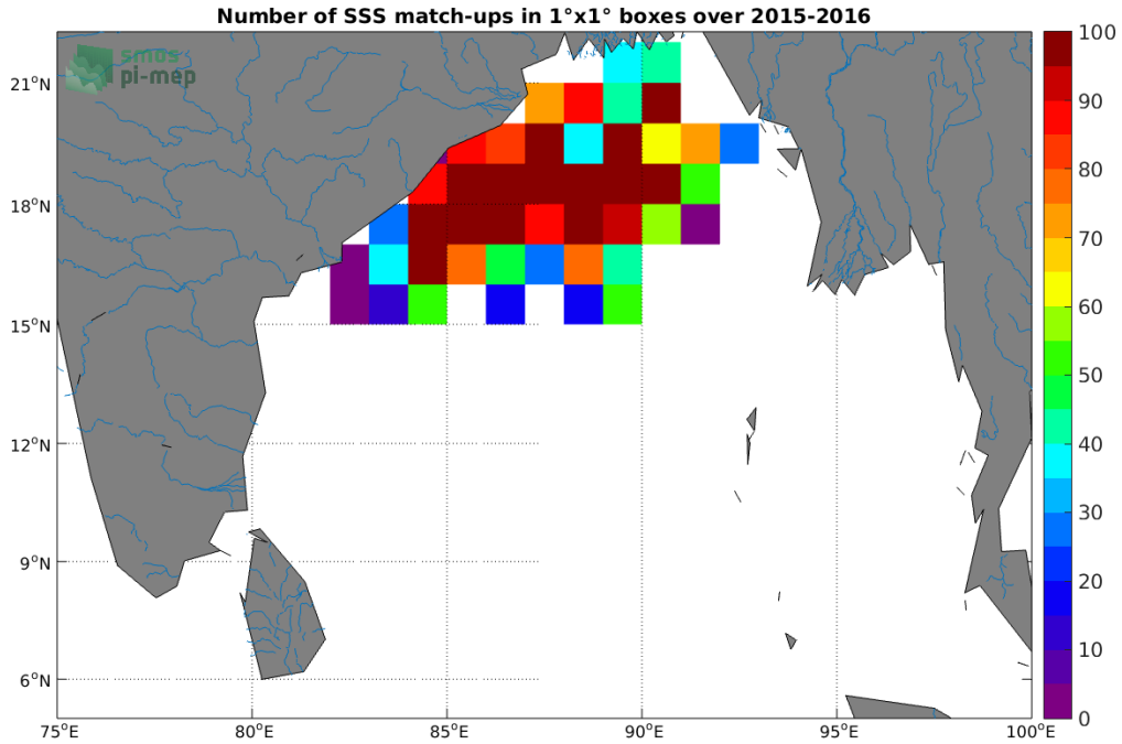
Figure 3: Number of SSS match-ups between Surface drifters SSS and the SMAP SSS L2 v5.0 (JPL) SSS product for the Ganga and Brahmaputra river plumes Pi-MEP region over 1^{\circ} \times 1^{\circ} boxes and for the full satellite product period.
