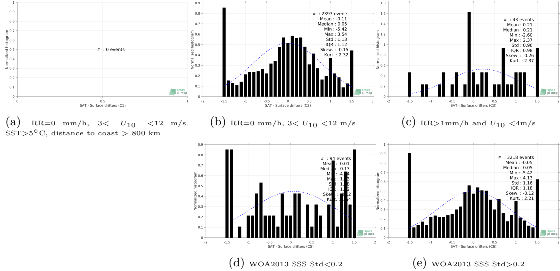
Figure 12: Normalized histogram of \Delta SSS (SMAP SSS L2 v5.0 (JPL) - Surface drifters) for 5 different subdatasets corresponding to: RR=0 mm/h, 3 < U_{10} < 12 m/s, SST>5°C, distance to coast > 800 km (a), RR=0 mm/h, 3 < U_{10} < 12 m/s (b), RR>1mm/h and U_{10} < 4 m/s (c), WOA2013 SSS Std<0.2 (d), WOA2013 SSS Std>0.2 (e).
