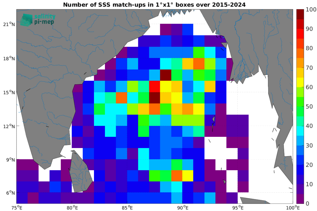
Figure 5: Number of SSS match-ups between Argo SSS and the SMAP SSS L2 v5.0 (JPL) SSS product for the Ganga and Brahmaputra river plumes Pi-MEP region over 1°x1° boxes and for the full satellite product period.
