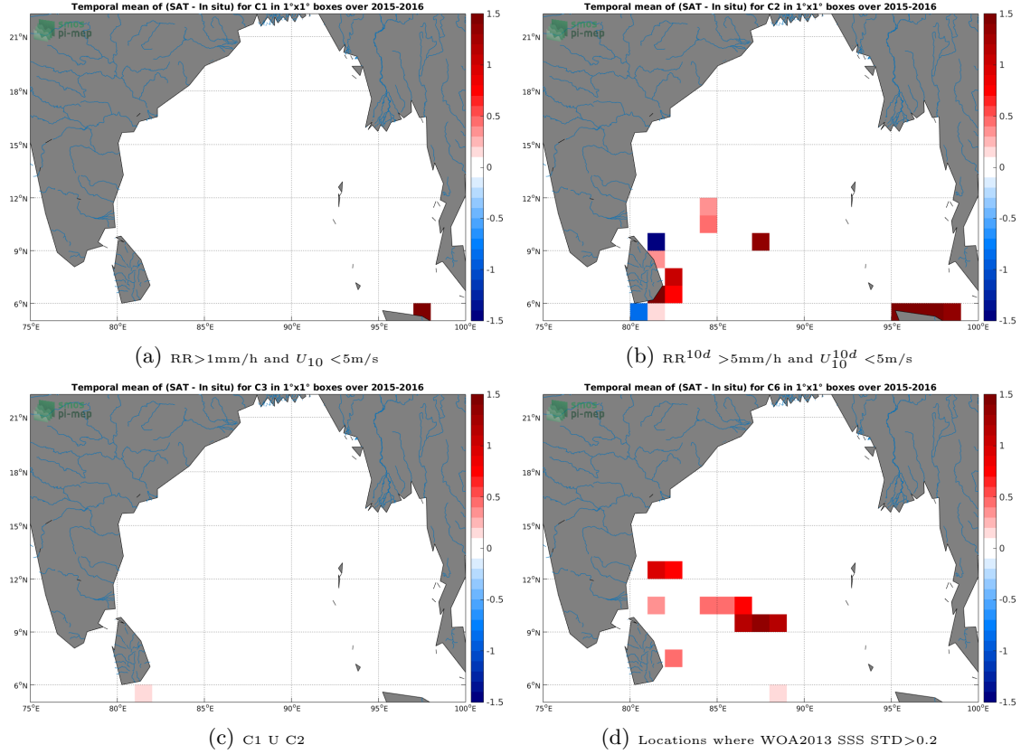
Figure 12: Temporal mean gridded over spatial boxes of size 1^\circ \times 1^\circ of \Delta SSS (SMAP-L2-JPL-V4 - TSG-LEGOS-DM) for 4 different subdatasets corresponding to: RR > 1\text{mm/h} and U_{10} < 5\text{m/s} (a), RR^{10d} > 5\text{mm/h} and U_{10}^{10d} < 5\text{m/s} (b), C1 U C2 (c), Locations where WOA2013 SSS STD > 0.2 (d).
