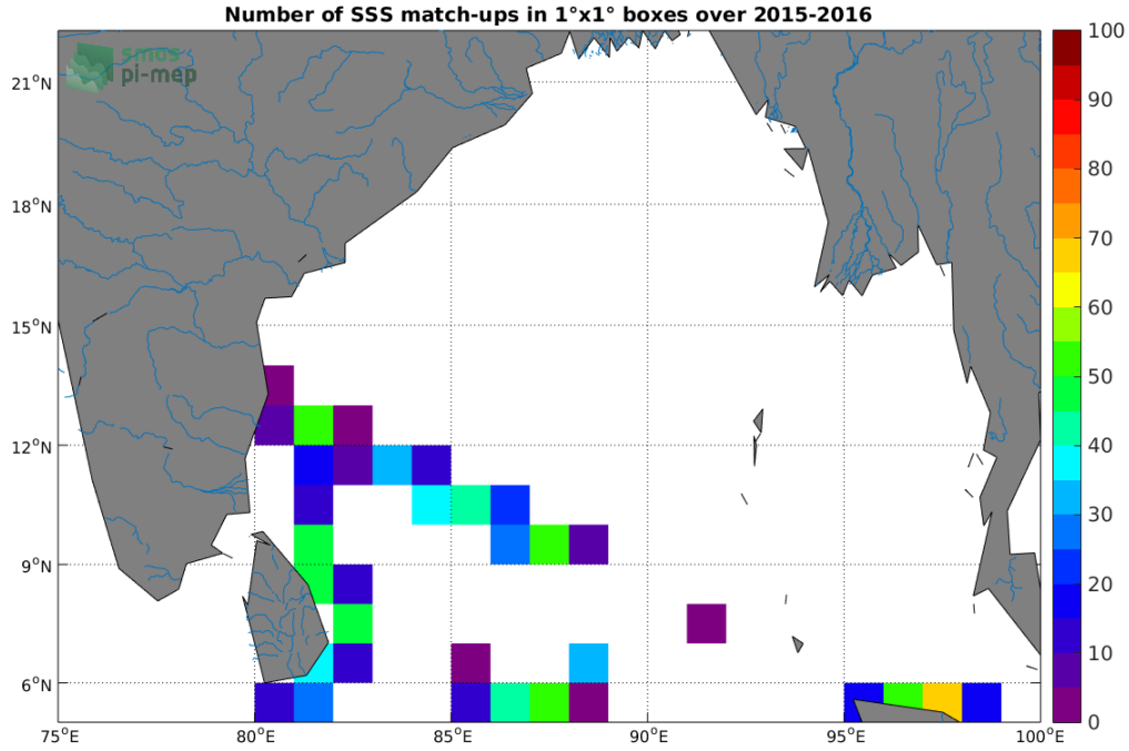
Figure 4: Number of SSS match-ups between TSG-LEGOS-DM SSS and the SMAP-L2-JPL-V4 SSS product for the Ganga and Brahmaputra river plumes Pi-MEP region over 1^\circ \times 1^\circ boxes and for the full satellite product period.
