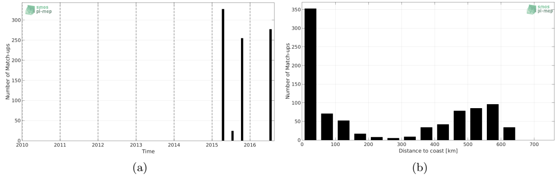
Figure 1: Number of match-ups between TSG-LEGOS-DM and SMAP-L2-JPL-V4 SSS as a function of time (a) and as function of the distance to coast (b) over the Ganga and Brahmaputra river plumes Pi-MEP region and for the full satellite product period.
