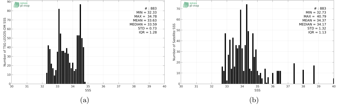
Figure 2: Histograms of SSS from TSG-LEGOS-DM (a) and SMAP-L2-JPL-V4 (b) considering all match-up pairs per bins of 0.1 over the Ganga and Brahmaputra river plumes Pi-MEP region and for the full satellite product period.
