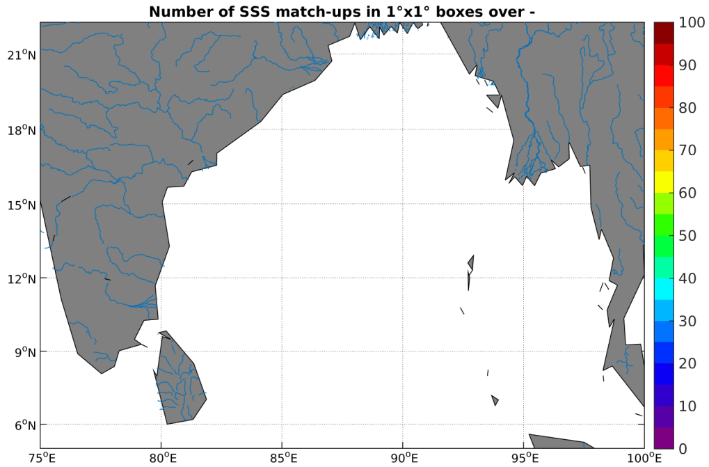
Figure 4: Number of SSS match-ups between TSG-GOSUD-Research-vessel SSS and the SMAP-L2-JPL-V4 SSS product for the Ganga and Brahmaputra river plumes Pi-MEP region over 1°x1° boxes and for the full satellite product period.
