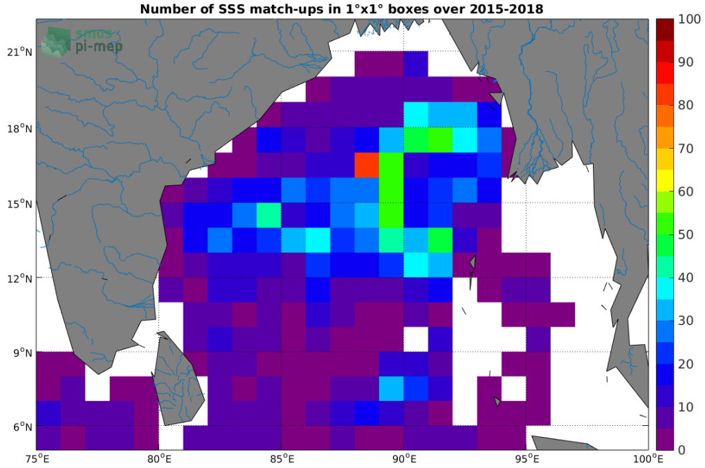
Figure 4: Number of SSS match-ups between Argo SSS and the SMAP-L2-JPL-V4 SSS product for the Ganga and Brahmaputra river plumes Pi-MEP region over 1°x1° boxes and for the full satellite product period.
