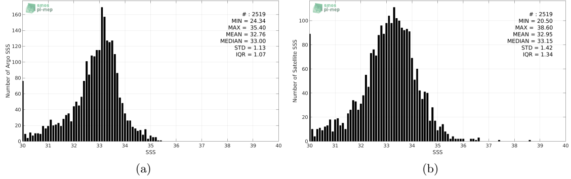
Figure 2: Histograms of SSS from Argo (a) and SMAP-L2-JPL-V4 (b) considering all match-up pairs per bins of 0.1 over the Ganga and Brahmaputra river plumes Pi-MEP region and for the full satellite product period.
