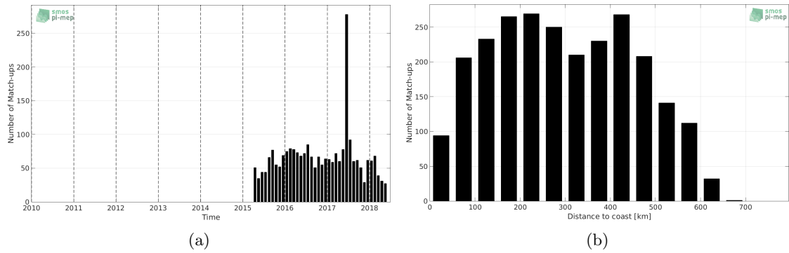
Figure 1: Number of match-ups between Argo and SMAP-L2-JPL-V4 SSS as a function of time (a) and as function of the distance to coast (b) over the Ganga and Brahmaputra river plumes Pi-MEP region and for the full satellite product period.
