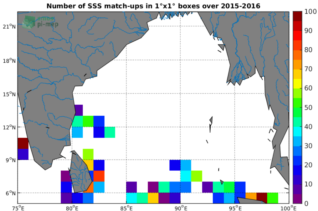
Figure 4: Number of SSS match-ups between TSG-LEGOS-DM SSS and the SMAP-L2-JPL-V4.2 SSS product for the Ganga and Brahmaputra river plumes Pi-MEP region over 1°x1° boxes and for the full satellite product period.
