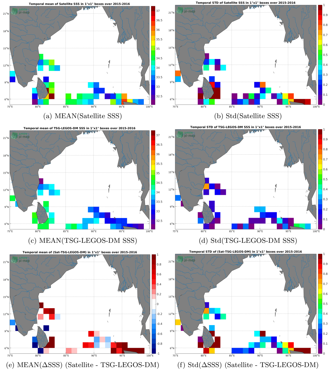
Figure 6: Temporal mean (left) and Std (right) of SSS from SMAP-L2-JPL-V4.2 (top), TSG-LEGOS-DM (middle), and of \Delta SSS (Satellite - TSG-LEGOS-DM). Only match-up pairs are used to generate these maps.
