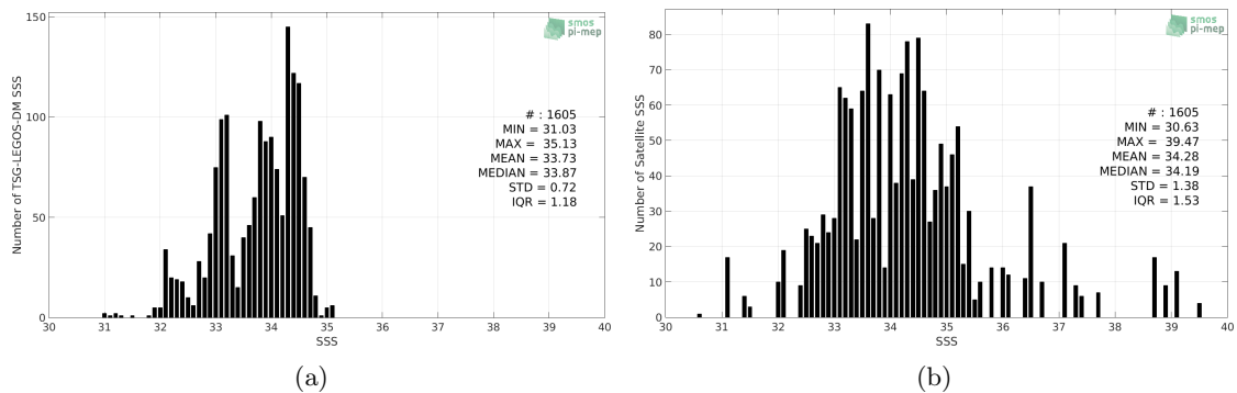
Figure 2: Histograms of SSS from TSG-LEGOS-DM (a) and SMAP-L2-JPL-V4.2 (b) considering all match-up pairs per bins of 0.1 over the Ganga and Brahmaputra river plumes Pi-MEP region and for the full satellite product period.
