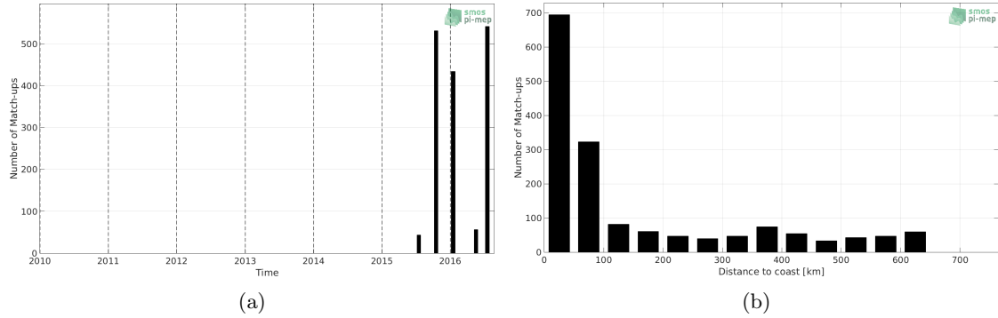
Figure 1: Number of match-ups between TSG-LEGOS-DM and SMAP-L2-JPL-V4.2 SSS as a function of time (a) and as function of the distance to coast (b) over the Ganga and Brahmaputra river plumes Pi-MEP region and for the full satellite product period.
