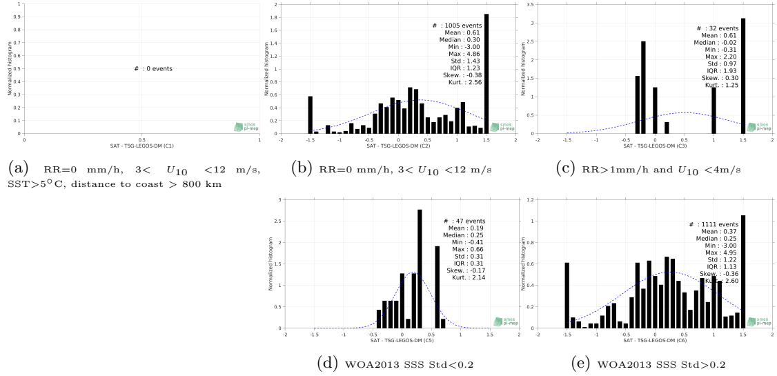
Figure 13: Normalized histogram of \Delta SSS (SMAP-L2-JPL-V4.2 - TSG-LEGOS-DM) for 5 different subdatasets corresponding to: RR=0 mm/h, 3 < U_{10} < 12 m/s, SST > 5°C, distance to coast > 800 km (a), RR=0 mm/h, 3 < U_{10} < 12 m/s (b), RR > 1mm/h and U_{10} < 4 m/s (c), WOA2013 SSS Std < 0.2 (d), WOA2013 SSS Std > 0.2 (e).
