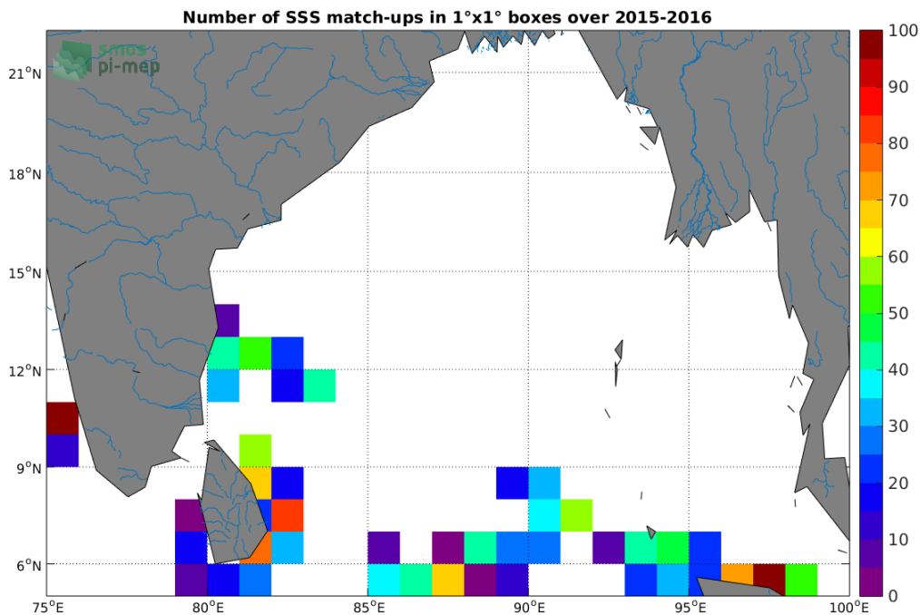
Figure 4: Number of SSS match-ups between TSG-LEGOS-DM SSS and the SMAP-L2-JPL-V4.2 SSS product for the Ganga and Brahmaputra river plumes Pi-MEP region over 1^\circ \times 1^\circ boxes and for the full satellite product period.
