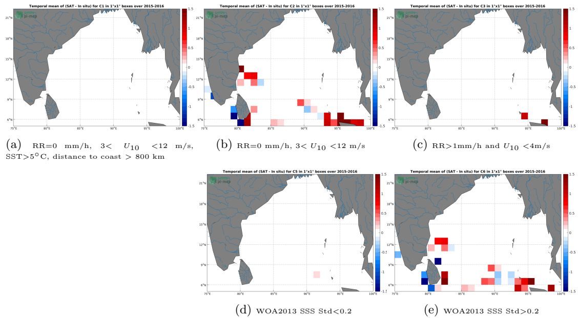
Figure 12: Temporal mean gridded over spatial boxes of size 1^\circ \times 1^\circ of \Delta SSS (SMAP-L2-JPL-V4.2 - TSG-LEGOS-DM) for 5 different subdatasets corresponding to:RR=0 mm/h, 3 < U_{10} < 12 m/s, SST >5^\circ C, distance to coast > 800 km (a), RR=0 mm/h, 3 < U_{10} < 12 m/s (b), RR >1 mm/h and U_{10} < 4 m/s (c), WOA2013 SSS Std <0.2 (d), WOA2013 SSS Std >0.2 (e).
