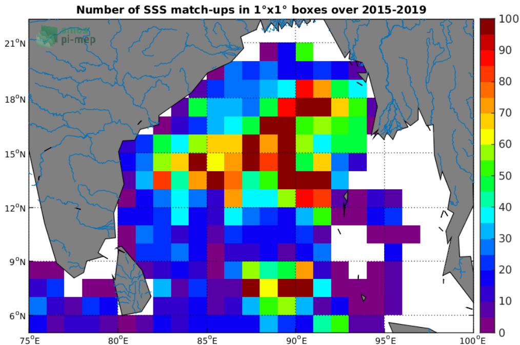
Figure 4: Number of SSS match-ups between Argos SSS and the SMAP-L2-JPL-V4.2 SSS product for the Ganga and Brahmaputra river plumes Pi-MEP region over 1°x1° boxes and for the full satellite product period.
