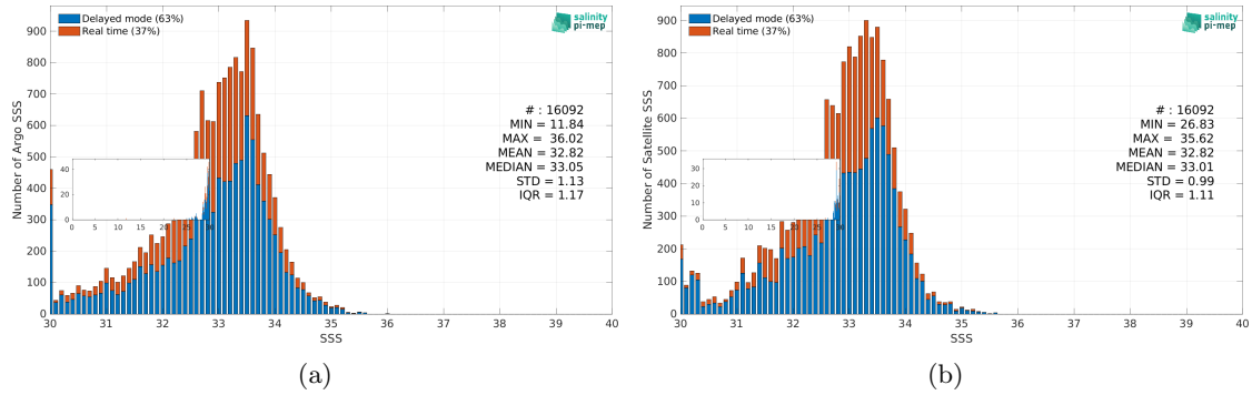
Figure 3: Histograms of SSS from Argo (a) and ISAS v7 - Monthly (Ifremer-LOPS-CMEMS) (b) considering all match-up pairs per bins of 0.1 over the Ganga and Brahmaputra river plumes Pi-MEP region and for the full satellite product period.
