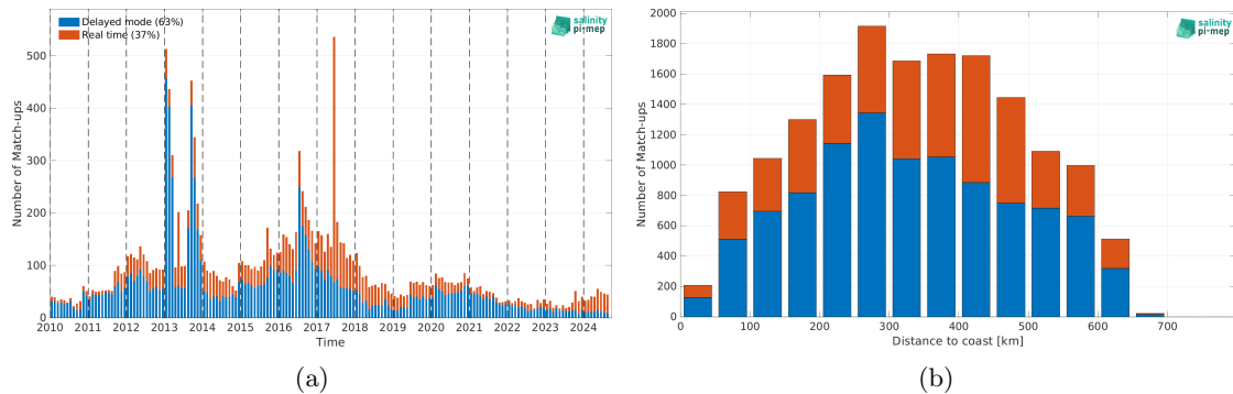
Figure 2: Number of match-ups between Argo and ISAS v7 - Monthly (Ifremer-LOPS-CMEMS) SSS as a function of time (a) and as function of the distance to coast (b) over the Ganga and Brahmaputra river plumes Pi-MEP region and for the full satellite product period.
