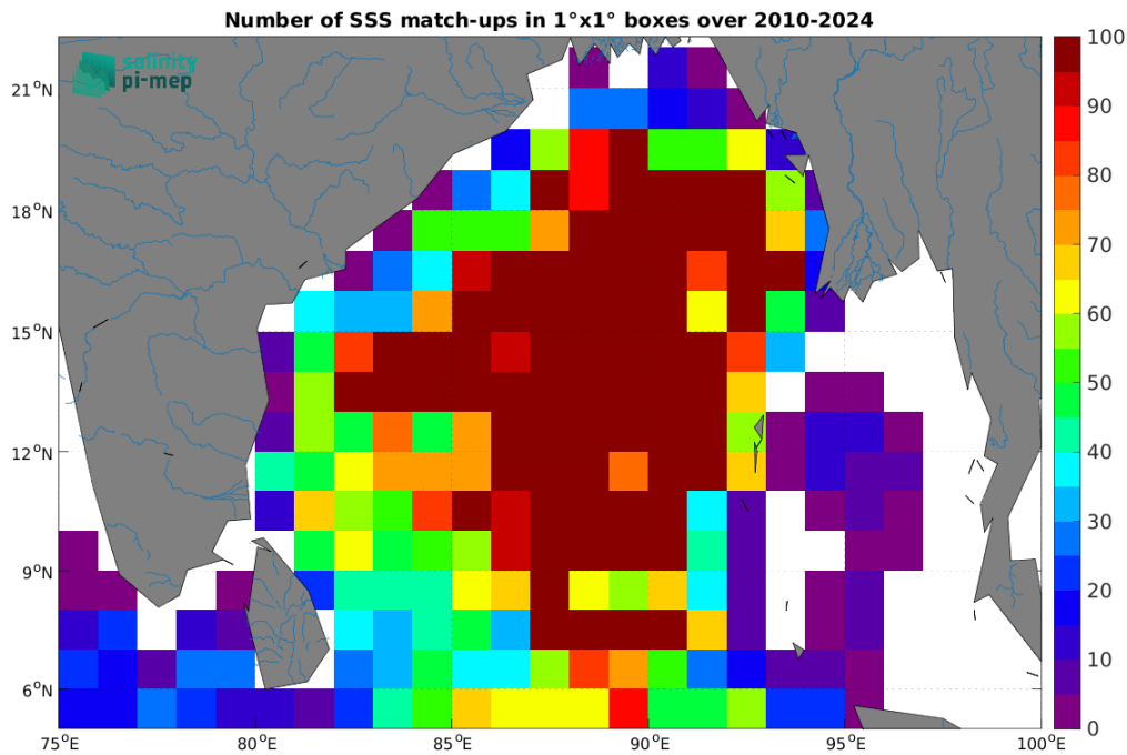
Figure 5: Number of SSS match-ups between Argo SSS and the ISAS v7 - Monthly (Ifremer-LOPS-CMEMS) SSS product for the Ganga and Brahmaputra river plumes Pi-MEP region over 1^\circ \times 1^\circ boxes and for the full satellite product period.
