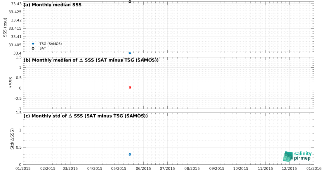
Figure 8: Time series of the monthly median SSS (top), median of \Delta SSS (Satellite - TSG (SAMOS)) and Std of \Delta SSS (Satellite - TSG (SAMOS)) over the Ganga and Brahmaputra river plumes Pi-MEP region considering all match-ups collected by the Pi-MEP.
