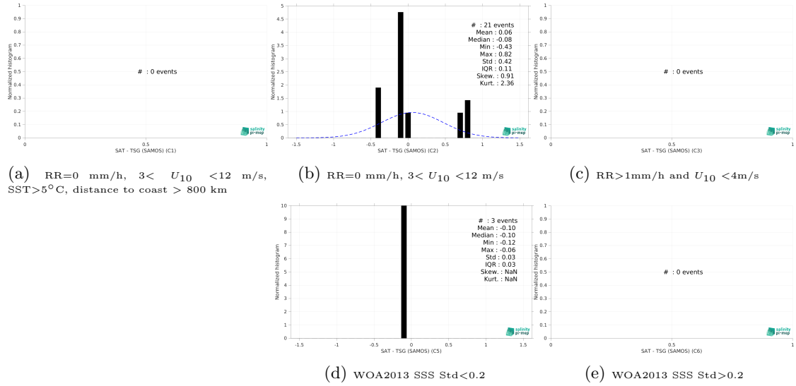
Figure 15: Normalized histogram of \Delta SSS (CCI SSS L4 Merged-OI v5.5 - 7-day running (ESA) - TSG (SAMOS)) for 5 different subdatasets corresponding to: RR=0 mm/h, 3 < U_{10} < 12 m/s, SST >5^{\circ}\text{C} , distance to coast > 800 km (a), RR=0 mm/h, 3 < U_{10} < 12 m/s (b), RR >1 mm/h and U_{10} < 4 m/s (c), WOA2013 SSS Std <0.2 (d), WOA2013 SSS Std >0.2 (e).
