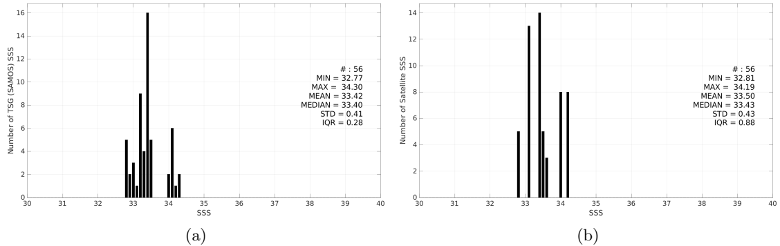
Figure 3: Histograms of SSS from TSG (SAMOS) (a) and CCI SSS L4 Merged-OI v5.5 - 7-day running (ESA) (b) considering all match-up pairs per bins of 0.1 over the Ganga and Brahmaputra river plumes Pi-MEP region and for the full satellite product period.
