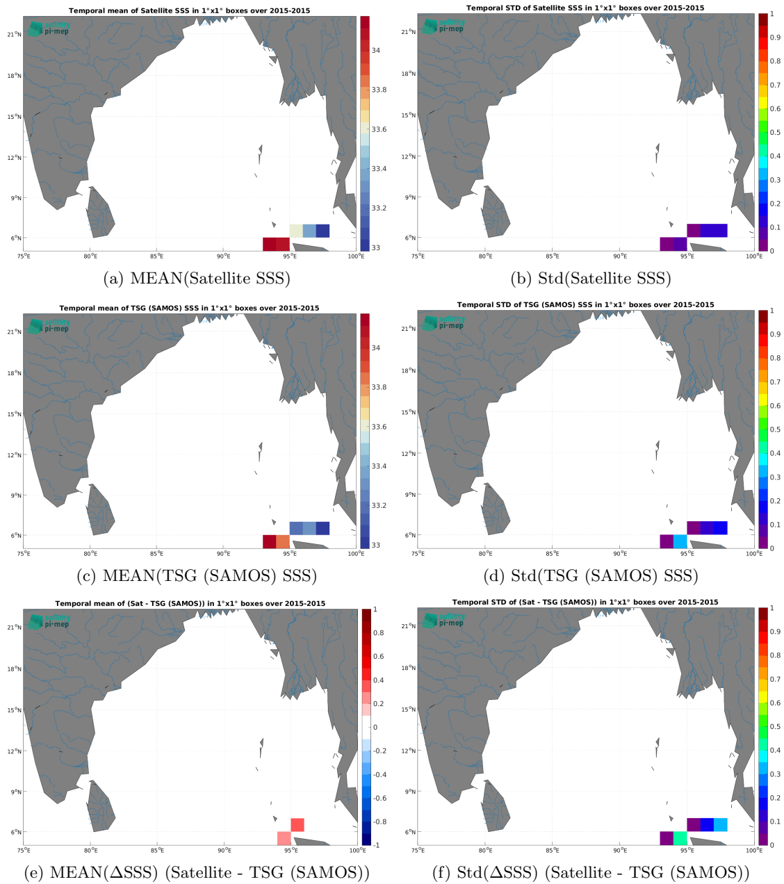
Figure 7: Temporal mean (left) and Std (right) of SSS from CCI SSS L4 Merged-OI v5.5 - 7-day running (ESA) (top), TSG (SAMOS) (middle), and of \Delta SSS (Satellite - TSG (SAMOS)). Only match-up pairs are used to generate these maps.
