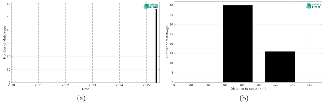
Figure 2: Number of match-ups between TSG (SAMOS) and CCI SSS L4 Merged-OI v5.5 - 7-day running (ESA) SSS as a function of time (a) and as function of the distance to coast (b) over the Ganga and Brahmaputra river plumes Pi-MEP region and for the full satellite product period.
