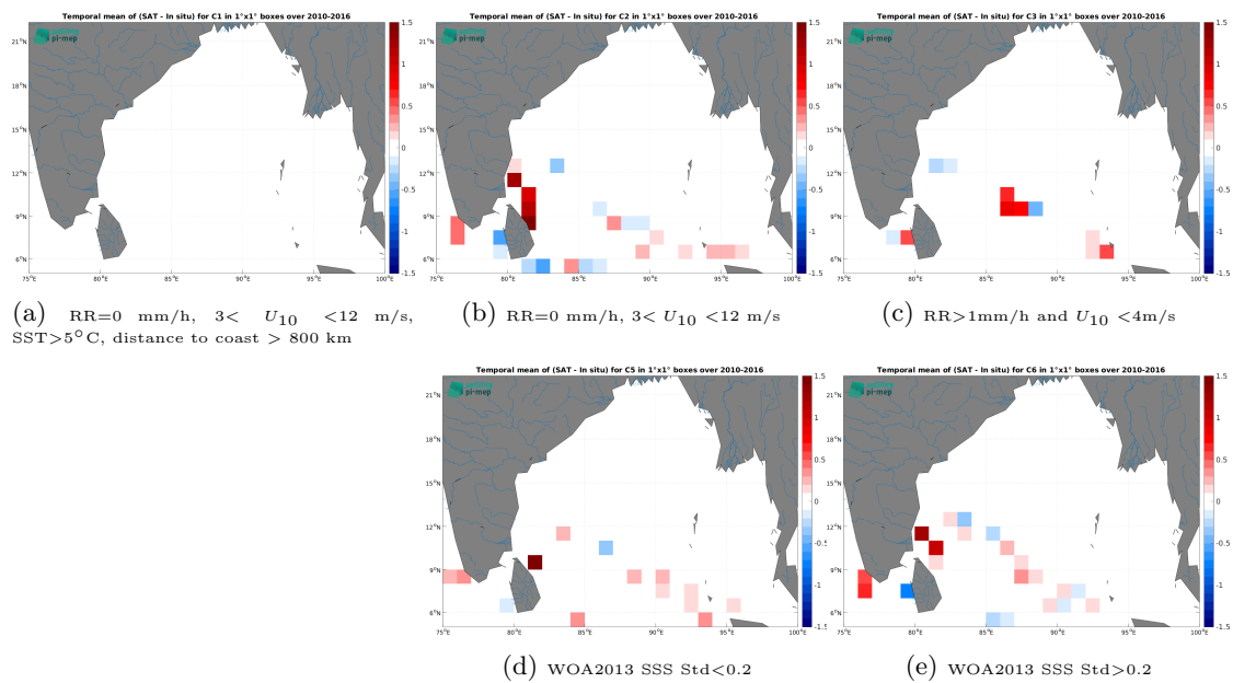
Figure 14: Temporal mean gridded over spatial boxes of size 1^\circ \times 1^\circ of \Delta SSS (CCI SSS L4 Merged-OI v5.5 - 7-day running (ESA) - TSG (LEGOS-DM)) for 5 different subdatasets corresponding to:RR=0 mm/h, 3 < U_{10} < 12 m/s, SST >5^\circ C, distance to coast > 800 km (a), RR=0 mm/h, 3 < U_{10} < 12 m/s (b), RR >1 mm/h and U_{10} < 4 m/s (c), WOA2013 SSS Std <0.2 (d), WOA2013 SSS Std >0.2 (e).
