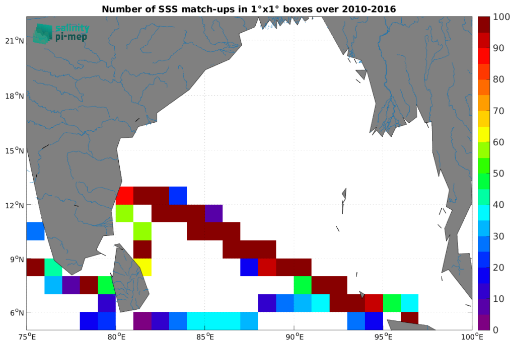
Figure 5: Number of SSS match-ups between TSG (LEGOS-DM) SSS and the CCI SSS L4 Merged-OI v5.5 - 7-day running (ESA) SSS product for the Ganga and Brahmaputra river plumes Pi-MEP region over 1^\circ \times 1^\circ boxes and for the full satellite product period.
