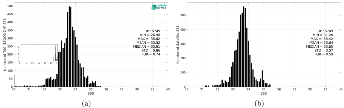
Figure 3: Histograms of SSS from TSG (LEGOS-DM) (a) and CCI SSS L4 Merged-OI v5.5 - 7-day running (ESA) (b) considering all match-up pairs per bins of 0.1 over the Ganga and Brahmaputra river plumes Pi-MEP region and for the full satellite product period.
