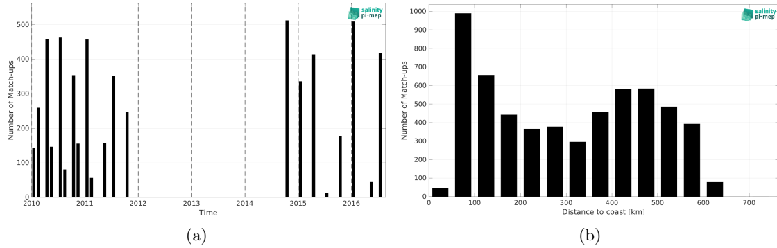
Figure 2: Number of match-ups between TSG (LEGOS-DM) and CCI SSS L4 Merged-OI v5.5 - 7-day running (ESA) SSS as a function of time (a) and as function of the distance to coast (b) over the Ganga and Brahmaputra river plumes Pi-MEP region and for the full satellite product period.
