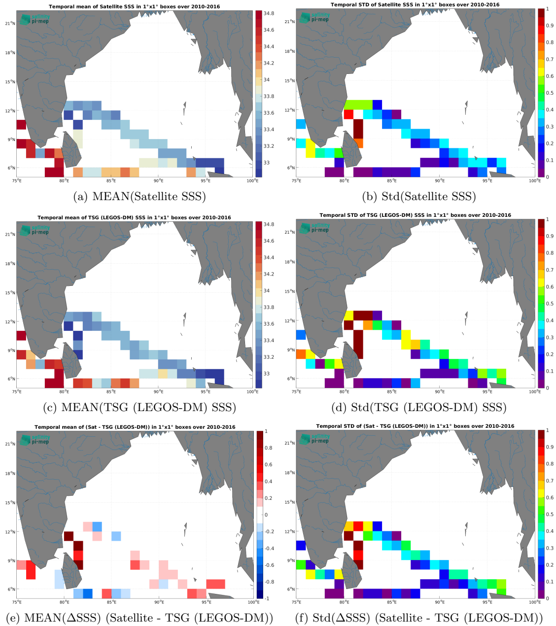
Figure 7: Temporal mean (left) and Std (right) of SSS from CCI SSS L4 Merged-OI v5.5 - 7-day running (ESA) (top), TSG (LEGOS-DM) (middle), and of \Delta SSS (Satellite - TSG (LEGOS-DM)). Only match-up pairs are used to generate these maps.
