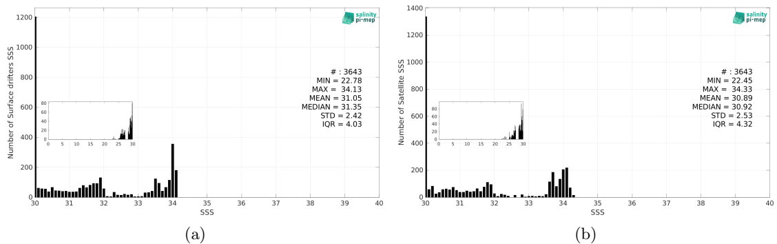
Figure 3: Histograms of SSS from Surface drifters (a) and CCI SSS L4 Merged-OI v5.5 - 7-day running (ESA) (b) considering all match-up pairs per bins of 0.1 over the Ganga and Brahmaputra river plumes Pi-MEP region and for the full satellite product period.
