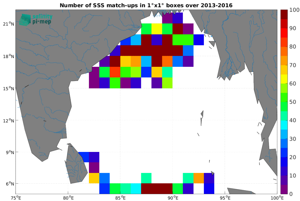
Figure 4: Number of SSS match-ups between Surface drifters SSS and the CCI SSS L4 Merged-OI v5.5 - 7-day running (ESA) SSS product for the Ganga and Brahmaputra river plumes Pi-MEP region over 1^\circ \times 1^\circ boxes and for the full satellite product period.
