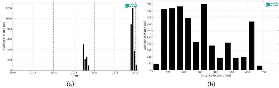
Figure 2: Number of match-ups between Surface drifters and CCI SSS L4 Merged-OI v5.5 - 7-day running (ESA) SSS as a function of time (a) and as function of the distance to coast (b) over the Ganga and Brahmaputra river plumes Pi-MEP region and for the full satellite product period.
