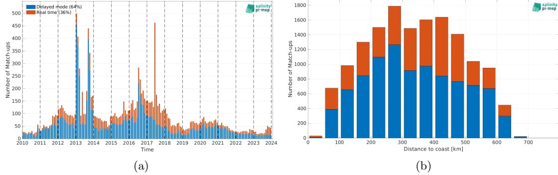
Figure 2: Number of match-ups between Argo and CCI SSS L4 Merged-OI v5.5 - 7-day running (ESA) SSS as a function of time (a) and as function of the distance to coast (b) over the Ganga and Brahmaputra river plumes Pi-MEP region and for the full satellite product period.
