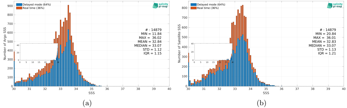
Figure 3: Histograms of SSS from Argo (a) and CCI SSS L4 Merged-OI v5.5 - 7-day running (ESA) (b) considering all match-up pairs per bins of 0.1 over the Ganga and Brahmaputra river plumes Pi-MEP region and for the full satellite product period.
