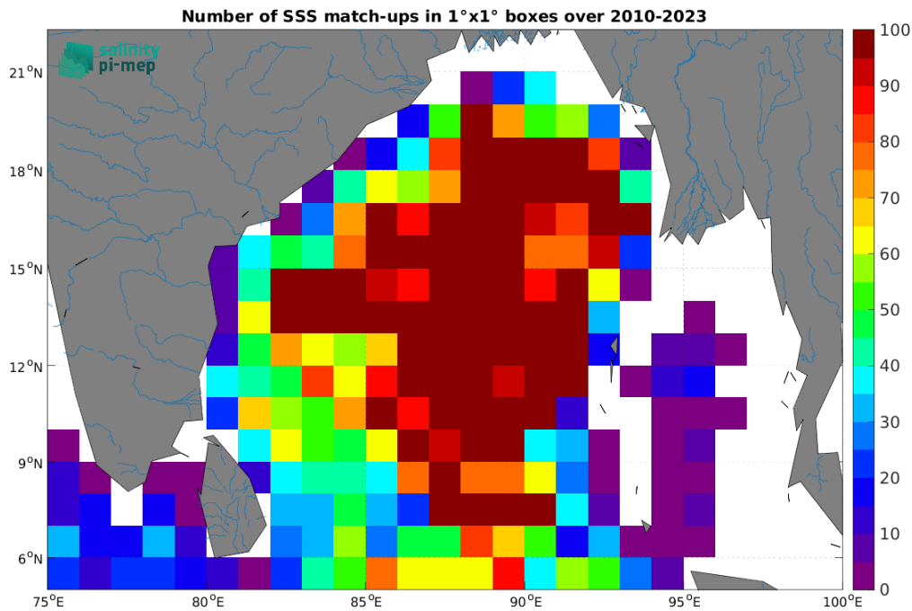
Figure 5: Number of SSS match-ups between Argo SSS and the CCI SSS L4 Merged-OI v5.5 - 7-day running (ESA) SSS product for the Ganga and Brahmaputra river plumes Pi-MEP region over 1^\circ \times 1^\circ boxes and for the full satellite product period.
