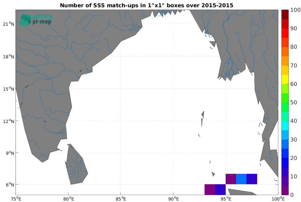
Figure 5: Number of SSS match-ups between TSG (SAMOS) SSS and the CCI SSS L4 Merged-OI v5.5 - 30-day running (ESA) SSS product for the Ganga and Brahmaputra river plumes Pi-MEP region over 1^\circ \times 1^\circ boxes and for the full satellite product period.
