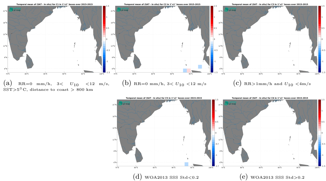
Figure 14: Temporal mean gridded over spatial boxes of size 1^\circ \times 1^\circ of \Delta SSS (CCI SSS L4 Merged-OI v5.5 - 30-day running (ESA) - TSG (SAMOS)) for 5 different subdatasets corresponding to:RR=0 mm/h, 3 < U_{10} < 12 m/s, SST >5^\circ C, distance to coast > 800 km (a), RR=0 mm/h, 3 < U_{10} < 12 m/s (b), RR >1 mm/h and U_{10} < 4 m/s (c), WOA2013 SSS Std <0.2 (d), WOA2013 SSS Std >0.2 (e).
