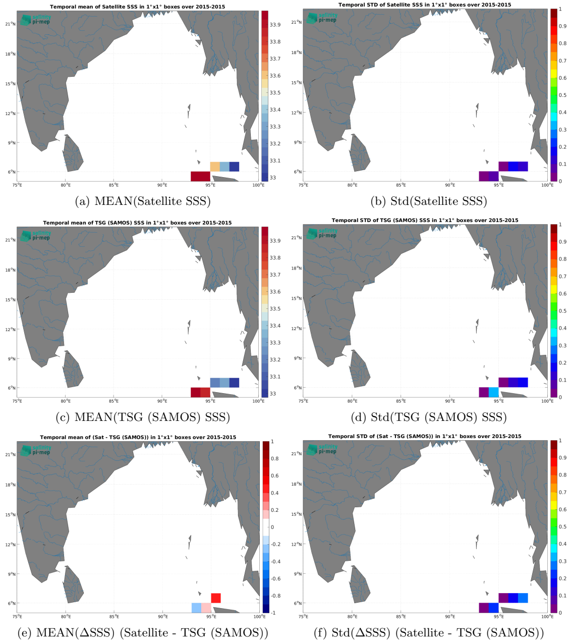
Figure 7: Temporal mean (left) and Std (right) of SSS from CCI SSS L4 Merged-OI v5.5 - 30-day running (ESA) (top), TSG (SAMOS) (middle), and of \Delta SSS (Satellite - TSG (SAMOS)). Only match-up pairs are used to generate these maps.
