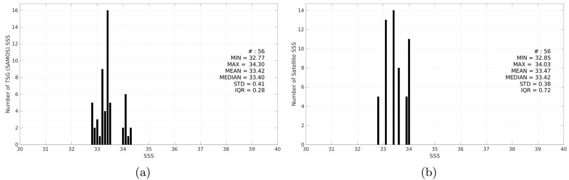
Figure 3: Histograms of SSS from TSG (SAMOS) (a) and CCI SSS L4 Merged-OI v5.5 - 30-day running (ESA) (b) considering all match-up pairs per bins of 0.1 over the Ganga and Brahmaputra river plumes Pi-MEP region and for the full satellite product period.
