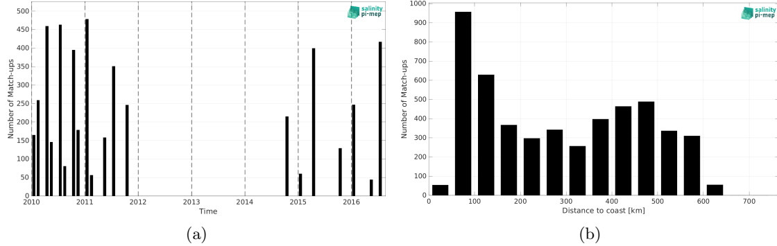
Figure 2: Number of match-ups between TSG (LEGOS-DM) and CCI SSS L4 Merged-OI v5.5 - 30-day running (ESA) SSS as a function of time (a) and as function of the distance to coast (b) over the Ganga and Brahmaputra river plumes Pi-MEP region and for the full satellite product period.
