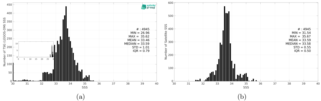
Figure 3: Histograms of SSS from TSG (LEGOS-DM) (a) and CCI SSS L4 Merged-OI v5.5 - 30-day running (ESA) (b) considering all match-up pairs per bins of 0.1 over the Ganga and Brahmaputra river plumes Pi-MEP region and for the full satellite product period.
