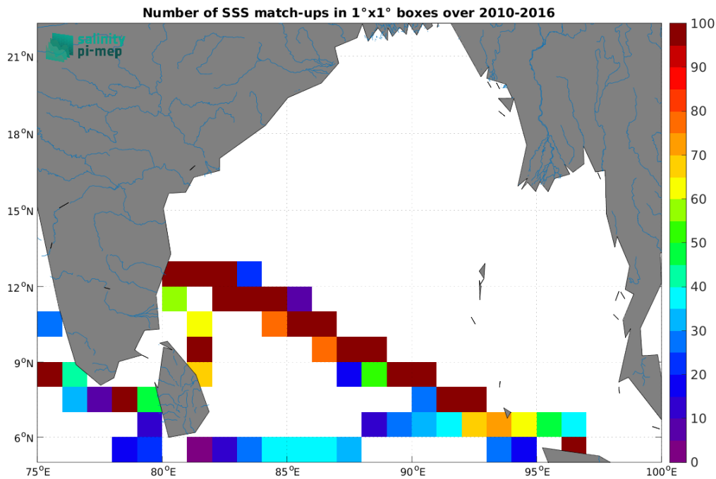
Figure 5: Number of SSS match-ups between TSG (LEGOS-DM) SSS and the CCI SSS L4 Merged-OI v5.5 - 30-day running (ESA) SSS product for the Ganga and Brahmaputra river plumes Pi-MEP region over 1^\circ \times 1^\circ boxes and for the full satellite product period.
