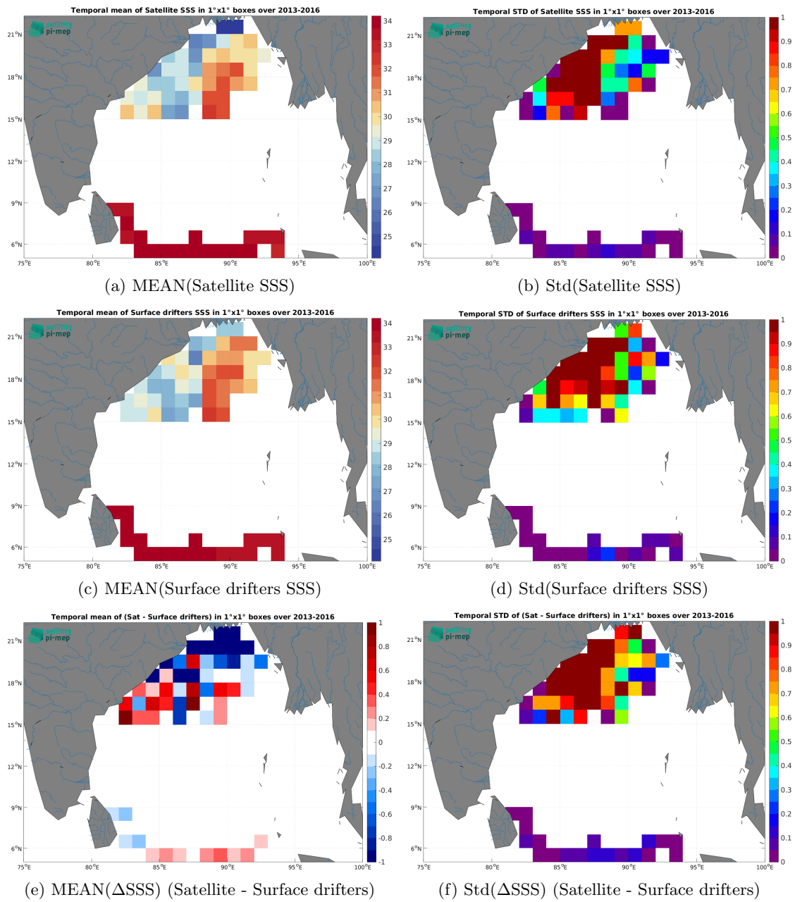
Figure 6: Temporal mean (left) and Std (right) of SSS from CCI SSS L4 Merged-OI v5.5 - 30-day running (ESA) (top), Surface drifters (middle), and of \Delta SSS (Satellite - Surface drifters). Only match-up pairs are used to generate these maps.
