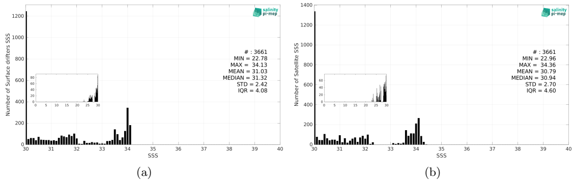
Figure 3: Histograms of SSS from Surface drifters (a) and CCI SSS L4 Merged-OI v5.5 - 30-day running (ESA) (b) considering all match-up pairs per bins of 0.1 over the Ganga and Brahmaputra river plumes Pi-MEP region and for the full satellite product period.
