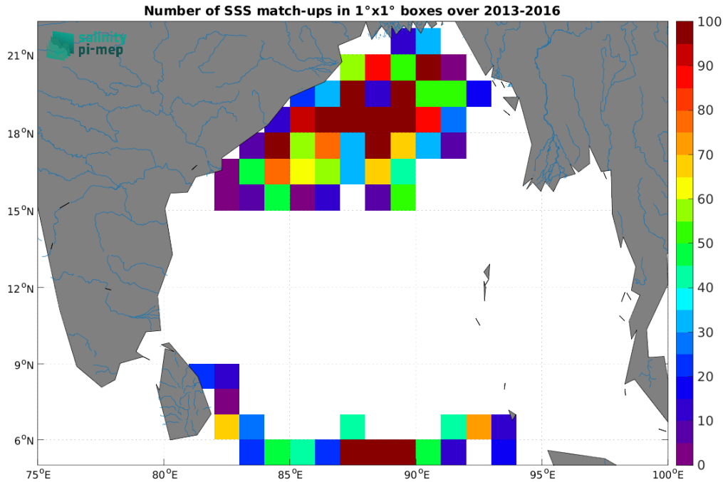
Figure 4: Number of SSS match-ups between Surface drifters SSS and the CCI SSS L4 Merged-OI v5.5 - 30-day running (ESA) SSS product for the Ganga and Brahmaputra river plumes Pi-MEP region over 1^{\circ} \times 1^{\circ} boxes and for the full satellite product period.
