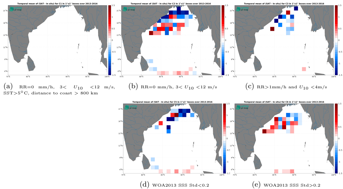
Figure 13: Temporal mean gridded over spatial boxes of size 1^\circ \times 1^\circ of \Delta SSS (CCI SSS L4 Merged-OI v5.5 - 30-day running (ESA) - Surface drifters) for 5 different subdatasets corresponding to:RR=0 mm/h, 3 < U_{10} < 12 m/s, SST >5^\circ C, distance to coast > 800 km (a), RR=0 mm/h, 3 < U_{10} < 12 m/s (b), RR >1 mm/h and U_{10} < 4 m/s (c), WOA2013 SSS Std <0.2 (d), WOA2013 SSS Std >0.2 (e).
