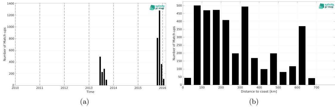
Figure 2: Number of match-ups between Surface drifters and CCI SSS L4 Merged-OI v5.5 - 30-day running (ESA) SSS as a function of time (a) and as function of the distance to coast (b) over the Ganga and Brahmaputra river plumes Pi-MEP region and for the full satellite product period.
