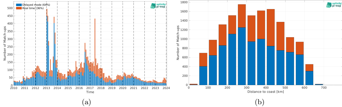
Figure 2: Number of match-ups between Argo and CCI SSS L4 Merged-OI v5.5 - 30-day running (ESA) SSS as a function of time (a) and as function of the distance to coast (b) over the Ganga and Brahmaputra river plumes Pi-MEP region and for the full satellite product period.
