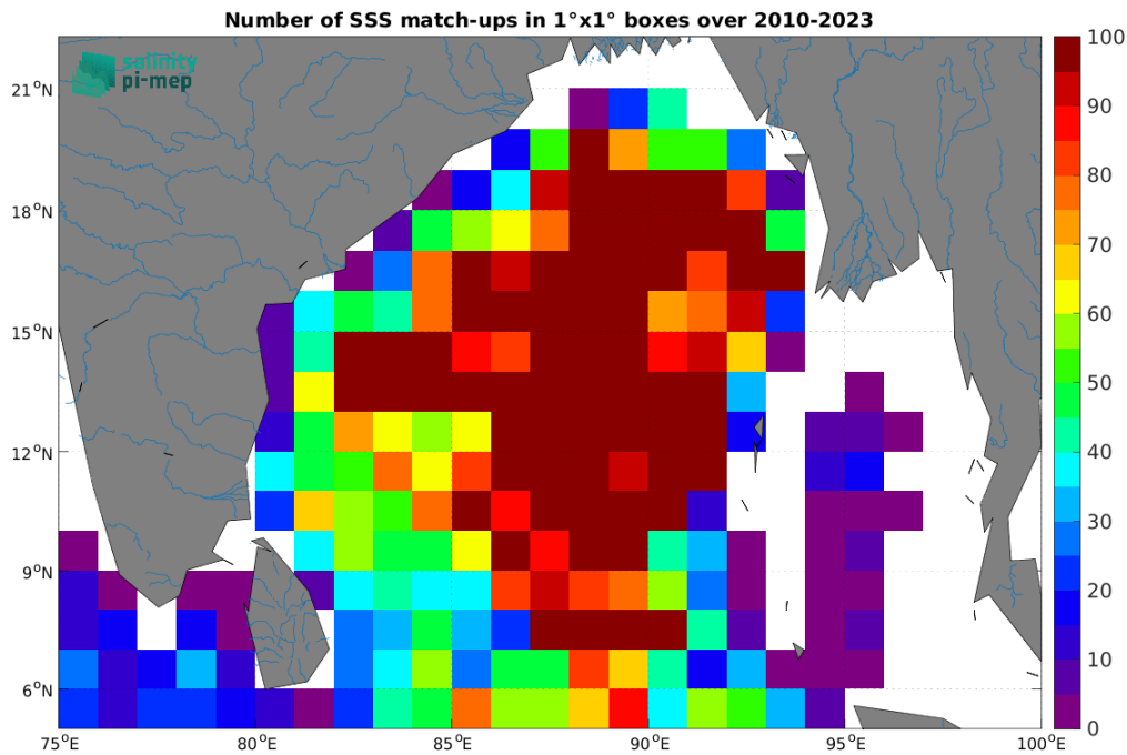
Figure 5: Number of SSS match-ups between Argo SSS and the CCI SSS L4 Merged-OI v5.5 - 30-day running (ESA) SSS product for the Ganga and Brahmaputra river plumes Pi-MEP region over 1^\circ \times 1^\circ boxes and for the full satellite product period.
