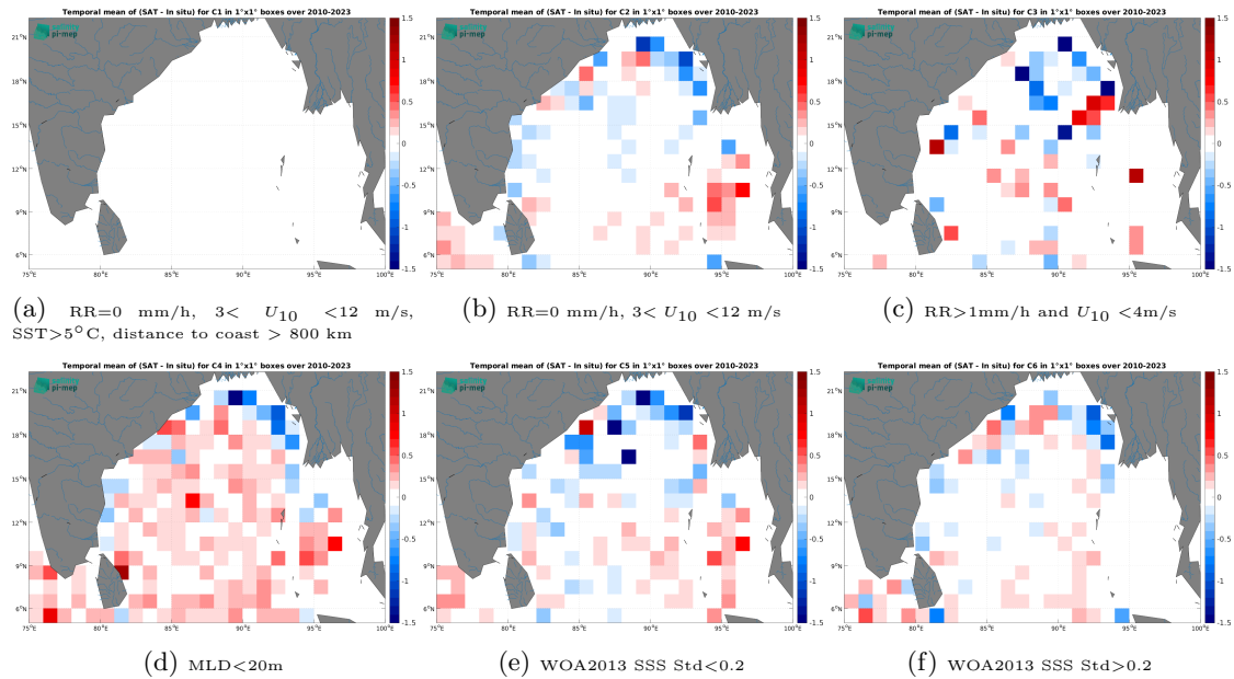
Figure 14: Temporal mean gridded over spatial boxes of size 1^\circ \times 1^\circ of \Delta SSS (CCI SSS L4 Merged-OI v5.5 - 30-day running (ESA) - Argo) for 6 different subdatasets corresponding to:RR=0 mm/h, 3 < U_{10} < 12 m/s, SST >5^\circ C, distance to coast > 800 km (a), RR=0 mm/h, 3 < U_{10} < 12 m/s (b), RR >1 mm/h and U_{10} < 4 m/s (c),MLD <20 m (d),WOA2013 SSS Std <0.2 (e),WOA2013 SSS Std >0.2 (f).
