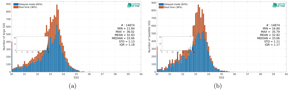
Figure 3: Histograms of SSS from Argo (a) and CCI SSS L4 Merged-OI v5.5 - 30-day running (ESA) (b) considering all match-up pairs per bins of 0.1 over the Ganga and Brahmaputra river plumes Pi-MEP region and for the full satellite product period.
