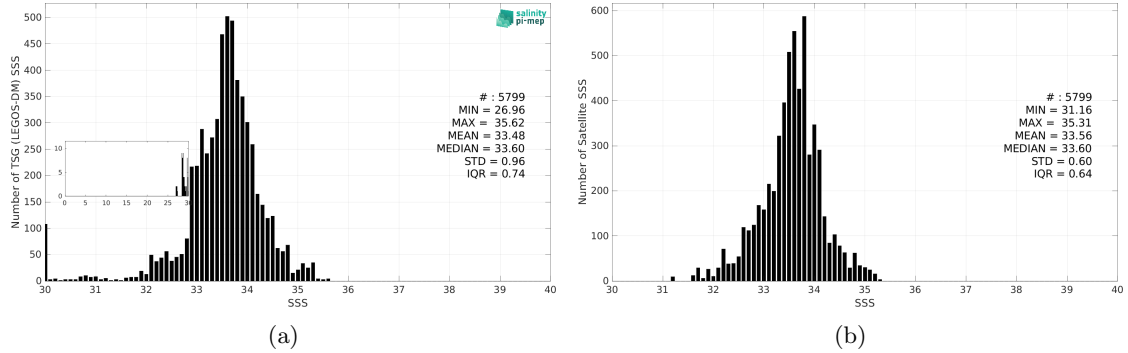
Figure 3: Histograms of SSS from TSG (LEGOS-DM) (a) and CCI SSS L4 Merged-OI v4.41 - 7-day running (ESA) (b) considering all match-up pairs per bins of 0.1 over the Ganga and Brahmaputra river plumes Pi-MEP region and for the full satellite product period.
