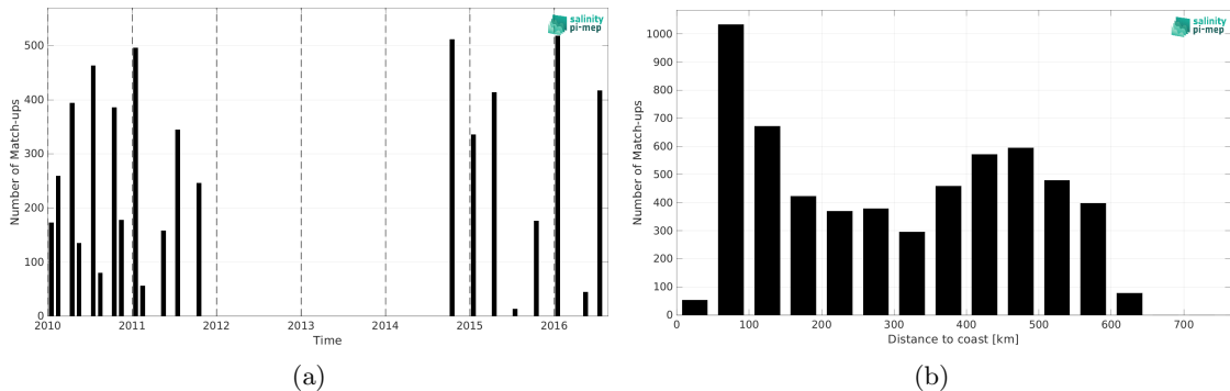
Figure 2: Number of match-ups between TSG (LEGOS-DM) and CCI SSS L4 Merged-OI v4.41 - 7-day running (ESA) SSS as a function of time (a) and as function of the distance to coast (b) over the Ganga and Brahmaputra river plumes Pi-MEP region and for the full satellite product period.
