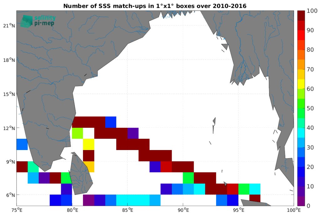
Figure 5: Number of SSS match-ups between TSG (LEGOS-DM) SSS and the CCI SSS L4 Merged-OI v4.41 - 7-day running (ESA) SSS product for the Ganga and Brahmaputra river plumes Pi-MEP region over 1^\circ \times 1^\circ boxes and for the full satellite product period.
