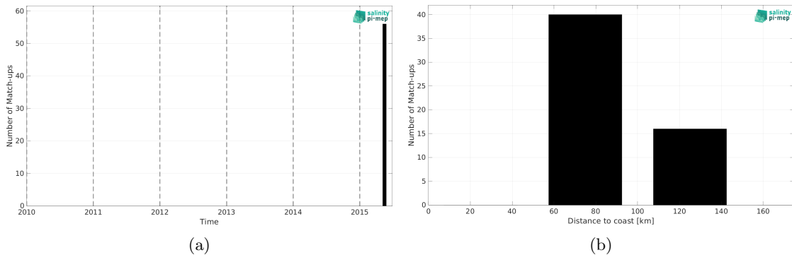
Figure 2: Number of match-ups between TSG (SAMOS) and CCI SSS L4 Merged-OI v4.41 - 30-day running (ESA) SSS as a function of time (a) and as function of the distance to coast (b) over the Ganga and Brahmaputra river plumes Pi-MEP region and for the full satellite product period.
