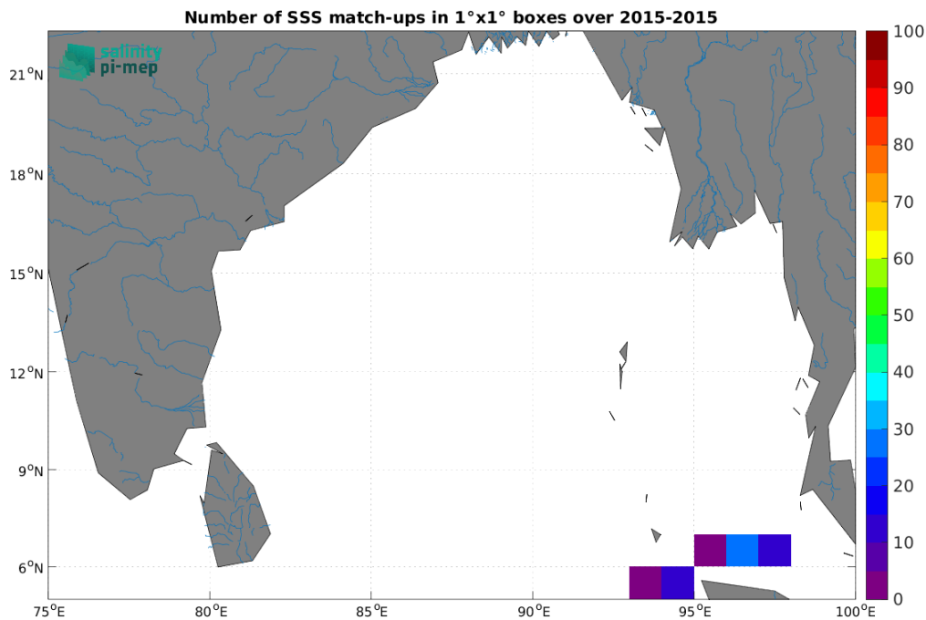
Figure 5: Number of SSS match-ups between TSG (SAMOS) SSS and the CCI SSS L4 Merged-OI v4.41 - 30-day running (ESA) SSS product for the Ganga and Brahmaputra river plumes Pi-MEP region over 1^\circ \times 1^\circ boxes and for the full satellite product period.
