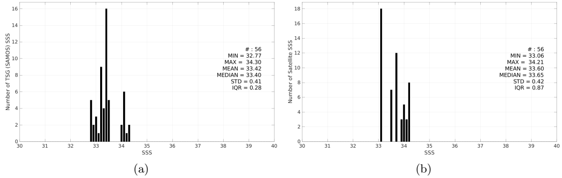
Figure 3: Histograms of SSS from TSG (SAMOS) (a) and CCI SSS L4 Merged-OI v4.41 - 30-day running (ESA) (b) considering all match-up pairs per bins of 0.1 over the Ganga and Brahmaputra river plumes Pi-MEP region and for the full satellite product period.
