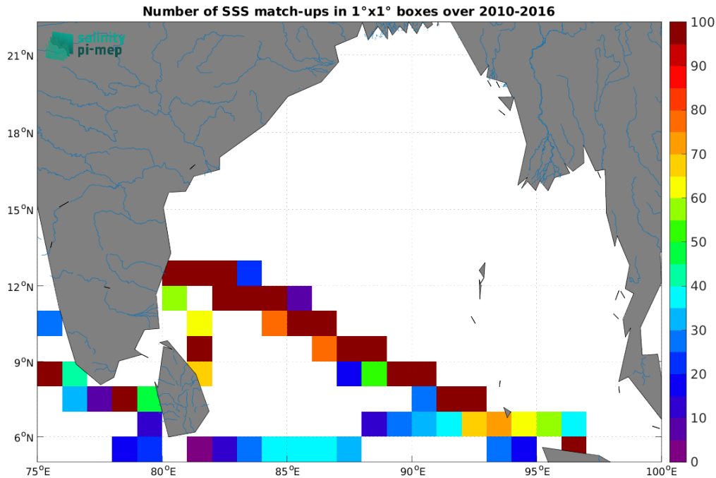
Figure 5: Number of SSS match-ups between TSG (LEGOS-DM) SSS and the CCI SSS L4 Merged-OI v4.41 - 30-day running (ESA) SSS product for the Ganga and Brahmaputra river plumes Pi-MEP region over 1^\circ \times 1^\circ boxes and for the full satellite product period.
