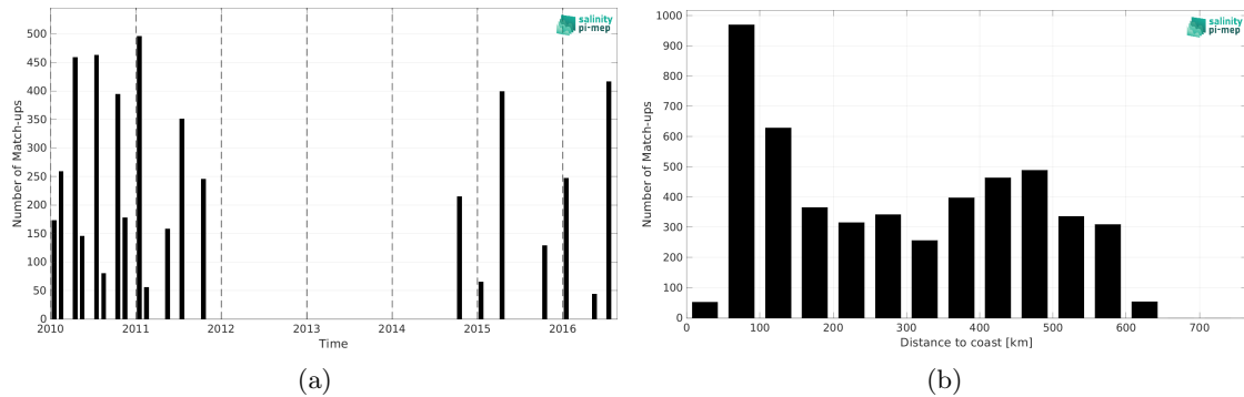
Figure 2: Number of match-ups between TSG (LEGOS-DM) and CCI SSS L4 Merged-OI v4.41 - 30-day running (ESA) SSS as a function of time (a) and as function of the distance to coast (b) over the Ganga and Brahmaputra river plumes Pi-MEP region and for the full satellite product period.
