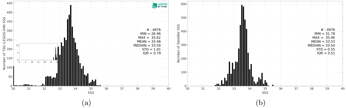
Figure 3: Histograms of SSS from TSG (LEGOS-DM) (a) and CCI SSS L4 Merged-OI v4.41 - 30-day running (ESA) (b) considering all match-up pairs per bins of 0.1 over the Ganga and Brahmaputra river plumes Pi-MEP region and for the full satellite product period.
