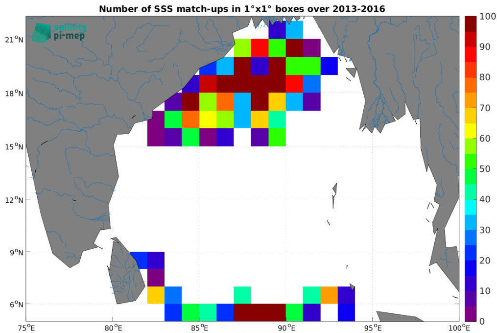
Figure 4: Number of SSS match-ups between Surface drifters SSS and the CCI SSS L4 Merged-OI v4.41 - 30-day running (ESA) SSS product for the Ganga and Brahmaputra river plumes Pi-MEP region over 1^\circ \times 1^\circ boxes and for the full satellite product period.
