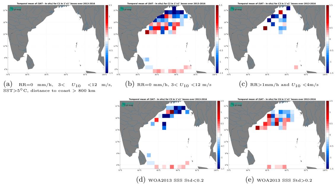
Figure 13: Temporal mean gridded over spatial boxes of size 1^\circ \times 1^\circ of \Delta SSS (CCI SSS L4 Merged-OI v4.41 - 30-day running (ESA) - Surface drifters) for 5 different subdatasets corresponding to:RR=0 mm/h, 3 < U_{10} < 12 m/s, SST >5^\circ C, distance to coast > 800 km (a), RR=0 mm/h, 3 < U_{10} < 12 m/s (b), RR >1 mm/h and U_{10} < 4 m/s (c), WOA2013 SSS Std <0.2 (d), WOA2013 SSS Std >0.2 (e).
