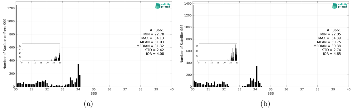
Figure 3: Histograms of SSS from Surface drifters (a) and CCI SSS L4 Merged-OI v4.41 - 30-day running (ESA) (b) considering all match-up pairs per bins of 0.1 over the Ganga and Brahmaputra river plumes Pi-MEP region and for the full satellite product period.
