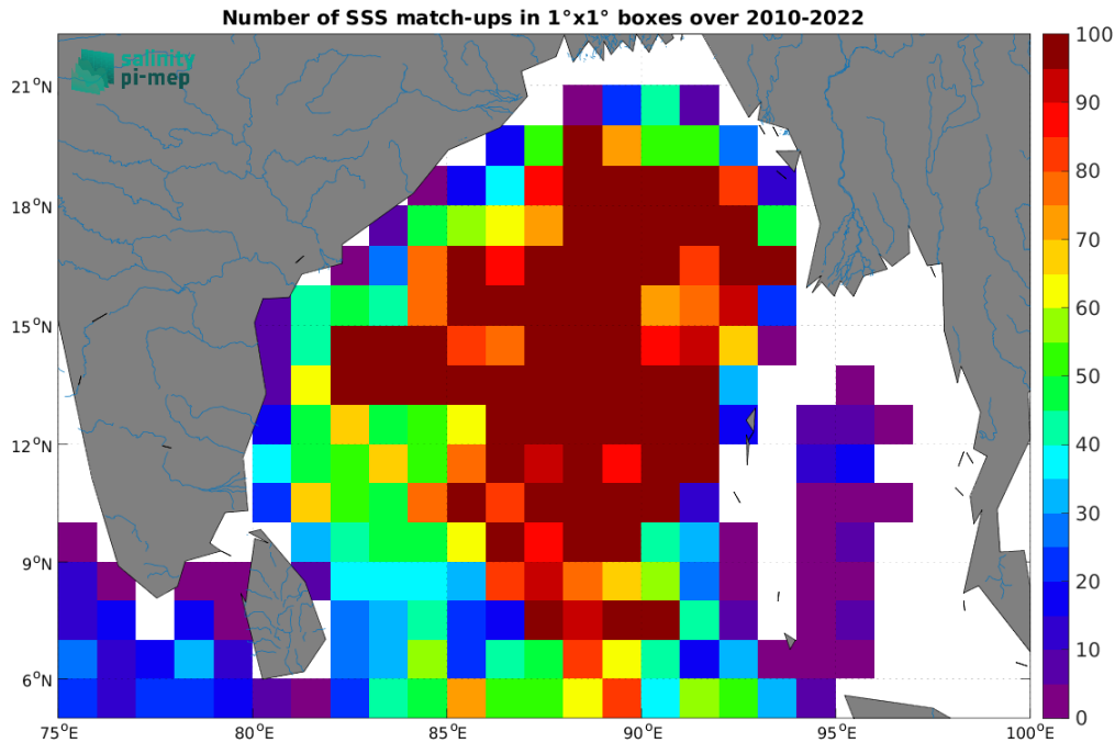
Figure 5: Number of SSS match-ups between Argo SSS and the CCI SSS L4 Merged-OI v4.41 - 30-day running (ESA) SSS product for the Ganga and Brahmaputra river plumes Pi-MEP region over 1^\circ \times 1^\circ boxes and for the full satellite product period.
