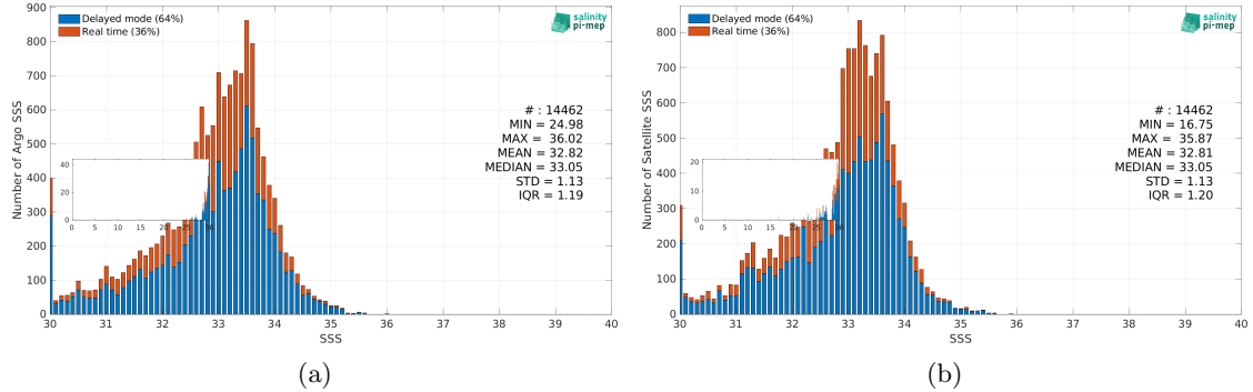
Figure 3: Histograms of SSS from Argo (a) and CCI SSS L4 Merged-OI v4.41 - 30-day running (ESA) (b) considering all match-up pairs per bins of 0.1 over the Ganga and Brahmaputra river plumes Pi-MEP region and for the full satellite product period.
