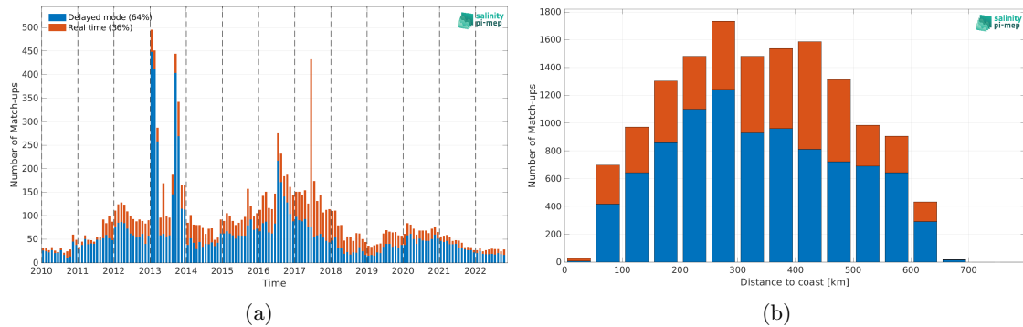
Figure 2: Number of match-ups between Argo and CCI SSS L4 Merged-OI v4.41 - 30-day running (ESA) SSS as a function of time (a) and as function of the distance to coast (b) over the Ganga and Brahmaputra river plumes Pi-MEP region and for the full satellite product period.
