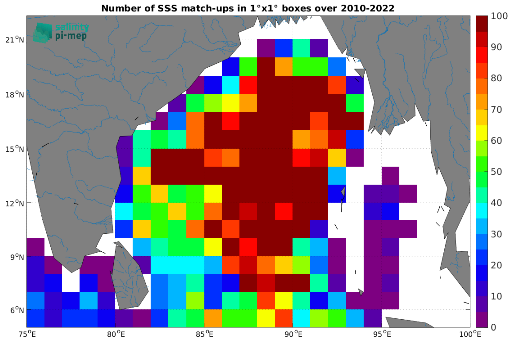
Figure 5: Number of SSS match-ups between Argo SSS and the CCI SSS L4 Merged-OI v4.41 - 30-day running (ESA) SSS product for the Ganga and Brahmaputra river plumes Pi-MEP region over 1^{\circ} \times 1^{\circ} boxes and for the full satellite product period.
