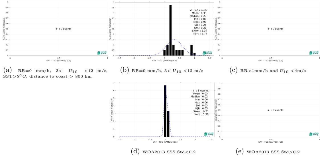
Figure 13: Normalized histogram of \Delta SSS (CCI SSS L4 Merged-OI v4.4 - 7-day running (ESA) - TSG (SAMOS)) for 5 different subdatasets corresponding to: RR=0 mm/h, 3 < U_{10} < 12 m/s, SST >5^{\circ} C, distance to coast > 800 km (a), RR=0 mm/h, 3 < U_{10} < 12 m/s (b), RR >1 mm/h and U_{10} < 4 m/s (c), WOA2013 SSS Std <0.2 (d), WOA2013 SSS Std >0.2 (e).
