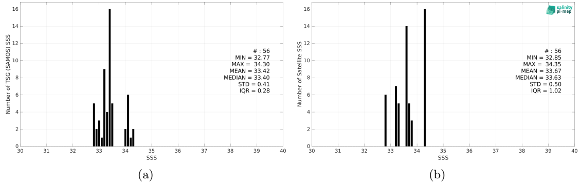
Figure 2: Histograms of SSS from TSG (SAMOS) (a) and CCI SSS L4 Merged-OI v4.4 - 7-day running (ESA) (b) considering all match-up pairs per bins of 0.1 over the Ganga and Brahmaputra river plumes Pi-MEP region and for the full satellite product period.
