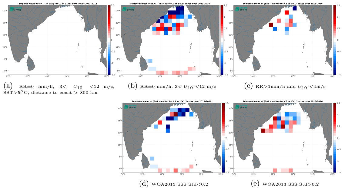
Figure 11: Temporal mean gridded over spatial boxes of size 1^\circ \times 1^\circ of \Delta SSS (CCI SSS L4 Merged-OI v4.4 - 30-day running (ESA) - Surface drifters) for 5 different subdatasets corresponding to:RR=0 mm/h, 3 < U_{10} < 12 m/s, SST >5^\circ\text{C} , distance to coast > 800 km (a), RR=0 mm/h, 3 < U_{10} < 12 m/s (b), RR >1 mm/h and U_{10} < 4 m/s (c), WOA2013 SSS Std <0.2 (d), WOA2013 SSS Std >0.2 (e).
