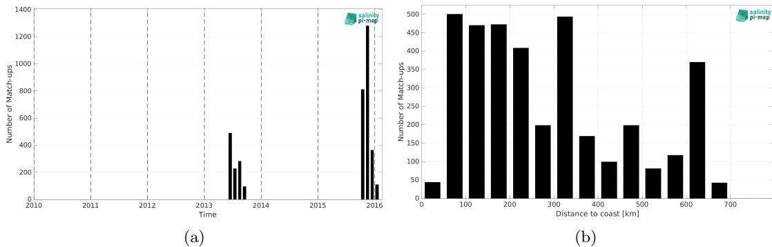
Figure 1: Number of match-ups between Surface drifters and CCI SSS L4 Merged-OI v4.4 - 30-day running (ESA) SSS as a function of time (a) and as function of the distance to coast (b) over the Ganga and Brahmaputra river plumes Pi-MEP region and for the full satellite product period.
