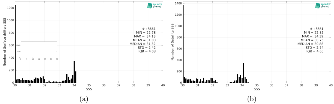
Figure 2: Histograms of SSS from Surface drifters (a) and CCI SSS L4 Merged-OI v4.4 - 30-day running (ESA) (b) considering all match-up pairs per bins of 0.1 over the Ganga and Brahmaputra river plumes Pi-MEP region and for the full satellite product period.
