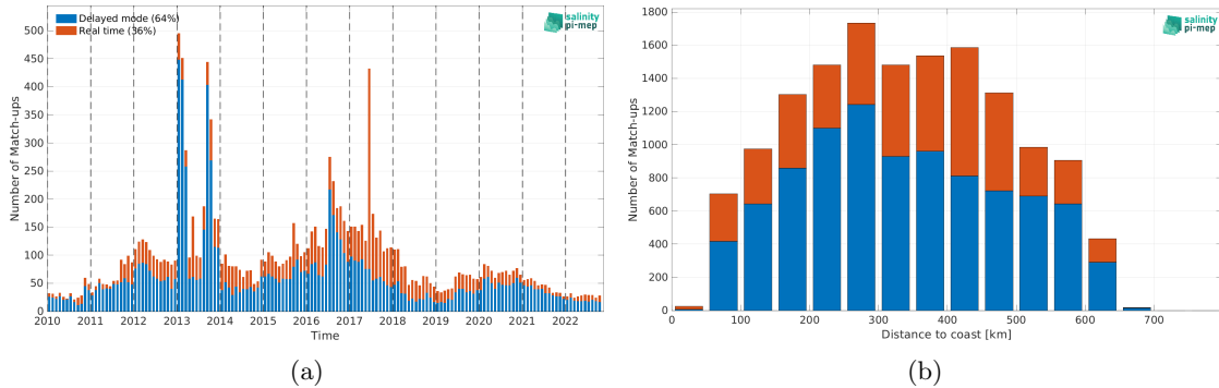
Figure 1: Number of match-ups between Argo and CCI SSS L4 Merged-OI v4.4 - 30-day running (ESA) SSS as a function of time (a) and as function of the distance to coast (b) over the Ganga and Brahmaputra river plumes Pi-MEP region and for the full satellite product period.
