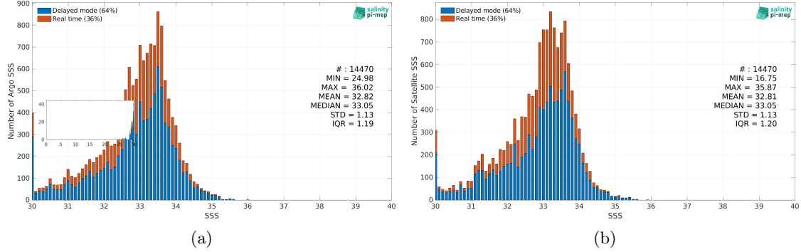
Figure 2: Histograms of SSS from Argo (a) and CCI SSS L4 Merged-OI v4.4 - 30-day running (ESA) (b) considering all match-up pairs per bins of 0.1 over the Ganga and Brahmaputra river plumes Pi-MEP region and for the full satellite product period.
