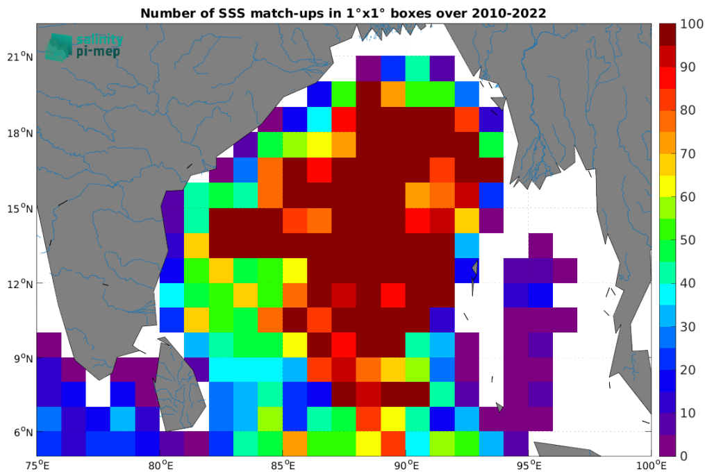
Figure 4: Number of SSS match-ups between Argo SSS and the CCI SSS L4 Merged-OI v4.4 - 30-day running (ESA) SSS product for the Ganga and Brahmaputra river plumes Pi-MEP region over 1^\circ \times 1^\circ boxes and for the full satellite product period.
