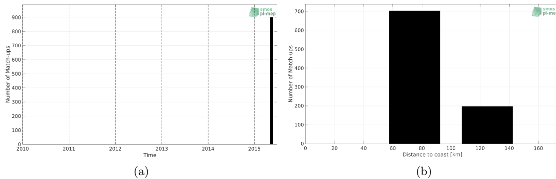
Figure 1: Number of match-ups between TSG (SAMOS) and CCI SSS L4 Merged-OI v3.2 - 7-day running (ESA) SSS as a function of time (a) and as function of the distance to coast (b) over the Ganga and Brahmaputra river plumes Pi-MEP region and for the full satellite product period.
