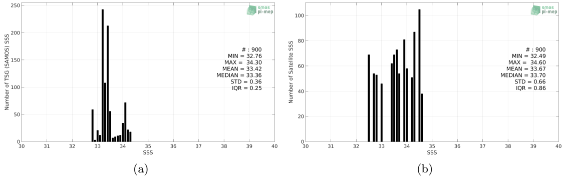
Figure 2: Histograms of SSS from TSG (SAMOS) (a) and CCI SSS L4 Merged-OI v3.2 - 7-day running (ESA) (b) considering all match-up pairs per bins of 0.1 over the Ganga and Brahmaputra river plumes Pi-MEP region and for the full satellite product period.
