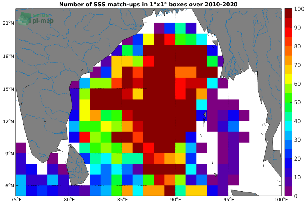
Figure 4: Number of SSS match-ups between Argo SSS and the CCI SSS L4 Merged-OI v3.2 - 7-day running (ESA) SSS product for the Ganga and Brahmaputra river plumes Pi-MEP region over 1^{\circ} \times 1^{\circ} boxes and for the full satellite product period.
