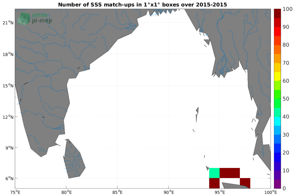
Figure 4: Number of SSS match-ups between TSG (SAMOS) SSS and the CCI SSS L4 Merged-OI v3.2 - 30-day running (ESA) SSS product for the Ganga and Brahmaputra river plumes Pi-MEP region over 1^\circ \times 1^\circ boxes and for the full satellite product period.
