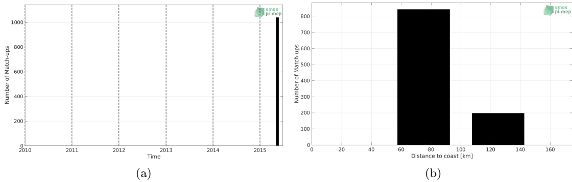
Figure 1: Number of match-ups between TSG (SAMOS) and CCI SSS L4 Merged-OI v3.2 - 30-day running (ESA) SSS as a function of time (a) and as function of the distance to coast (b) over the Ganga and Brahmaputra river plumes Pi-MEP region and for the full satellite product period.
