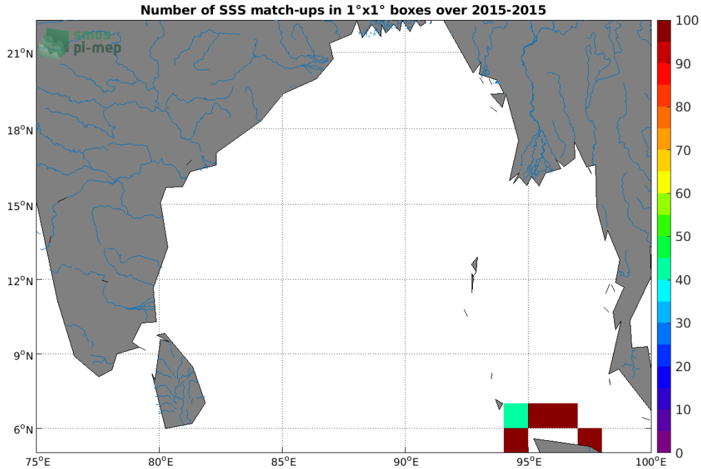
Figure 4: Number of SSS match-ups between TSG (SAMOS) SSS and the CCI SSS L4 Merged-OI v3.2 - 30-day running (ESA) SSS product for the Ganga and Brahmaputra river plumes Pi-MEP region over 1°x1° boxes and for the full satellite product period.
