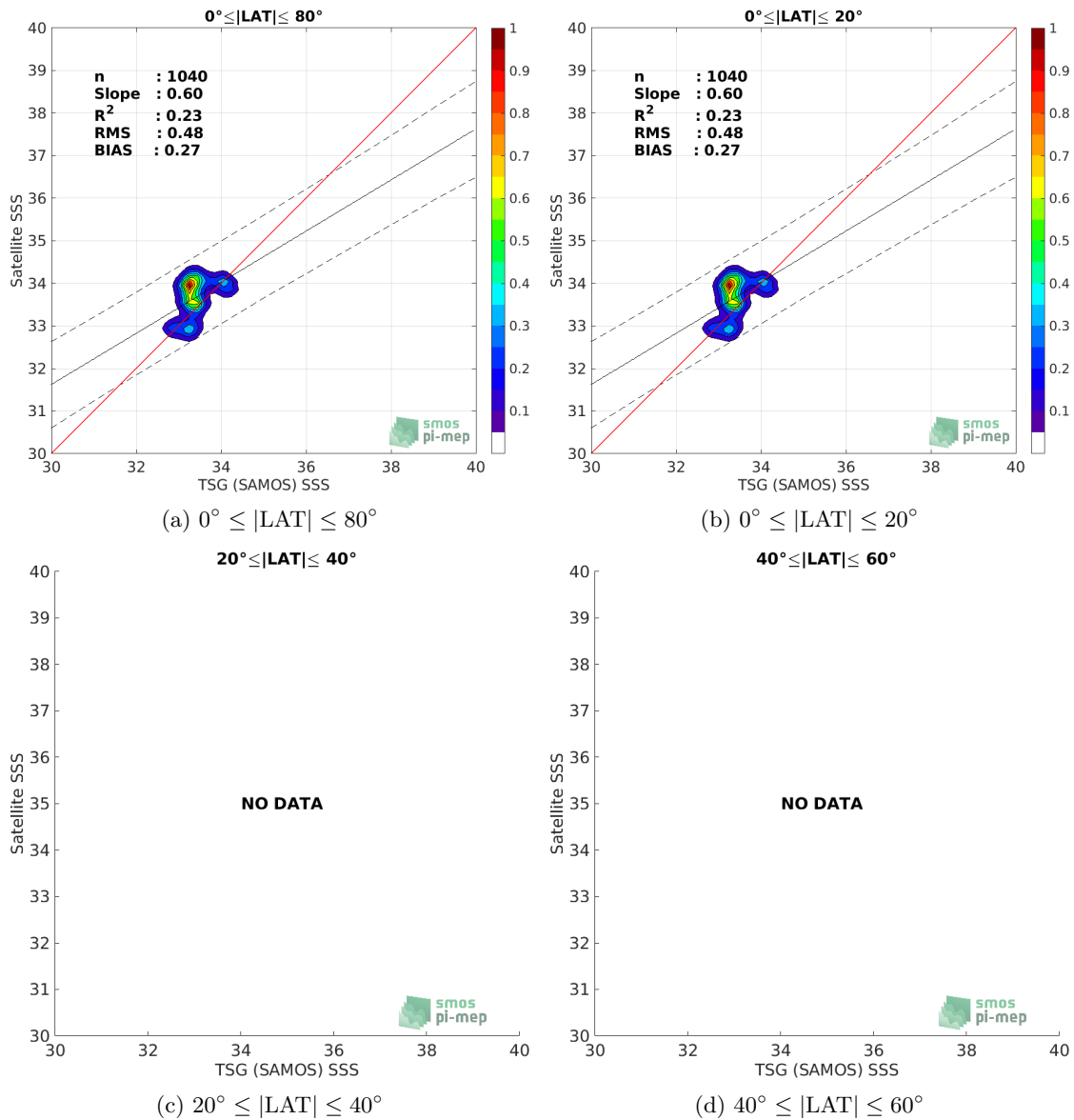
Figure 9: Contour maps of the concentration of CCI SSS L4 Merged-OI v3.2 - 30-day running (ESA) SSS ( y -axis) versus TSG (SAMOS) SSS ( x -axis) at match-up pairs for different latitude bands. For each plot, the red line shows x=y . The black thin and dashed lines indicate a linear fit through the data cloud and the \pm 95\% confidence levels, respectively. The number match-up pairs n , the slope and R^2 coefficient of the linear fit, the root mean square (RMS) and the mean bias between satellite and in situ data are indicated for each latitude band in each plots.
