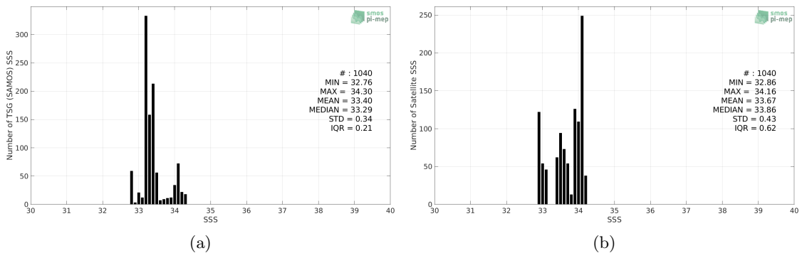
Figure 2: Histograms of SSS from TSG (SAMOS) (a) and CCI SSS L4 Merged-OI v3.2 - 30-day running (ESA) (b) considering all match-up pairs per bins of 0.1 over the Ganga and Brahmaputra river plumes Pi-MEP region and for the full satellite product period.
