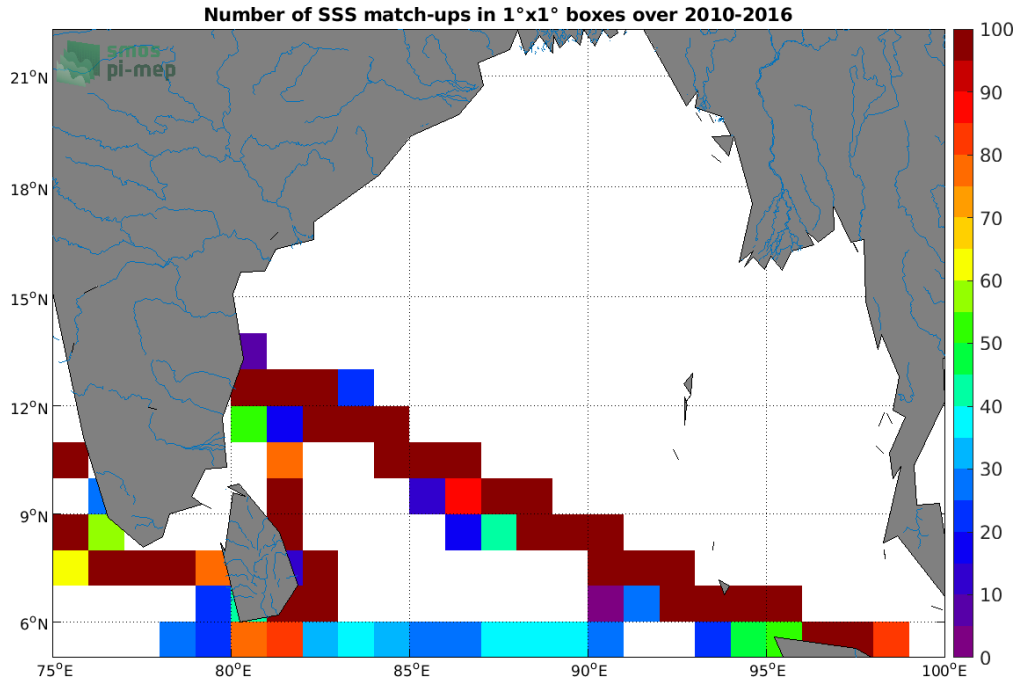
Figure 4: Number of SSS match-ups between TSG (LEGOS-DM) SSS and the CCI SSS L4 Merged-OI v3.2 - 30-day running (ESA) SSS product for the Ganga and Brahmaputra river plumes Pi-MEP region over 1°x1° boxes and for the full satellite product period.
