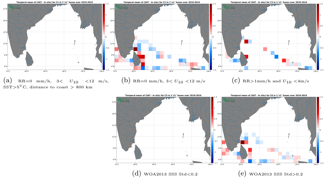
Figure 12: Temporal mean gridded over spatial boxes of size 1^{\circ}\times 1^{\circ} of \Delta\text{SSS} (CCI SSS L4 Merged-OI v3.2 - 30-day running (ESA) - TSG (LEGOS-DM)) for 5 different subdatasets corresponding to:RR=0 mm/h, 3 < U_{10} < 12 m/s, SST > 5^{\circ}\text{C} , distance to coast > 800 km (a), RR=0 mm/h, 3 < U_{10} < 12 m/s (b), RR > 1 mm/h and U_{10} < 4 m/s (c), WOA2013 SSS Std < 0.2 (d), WOA2013 SSS Std > 0.2 (e).
