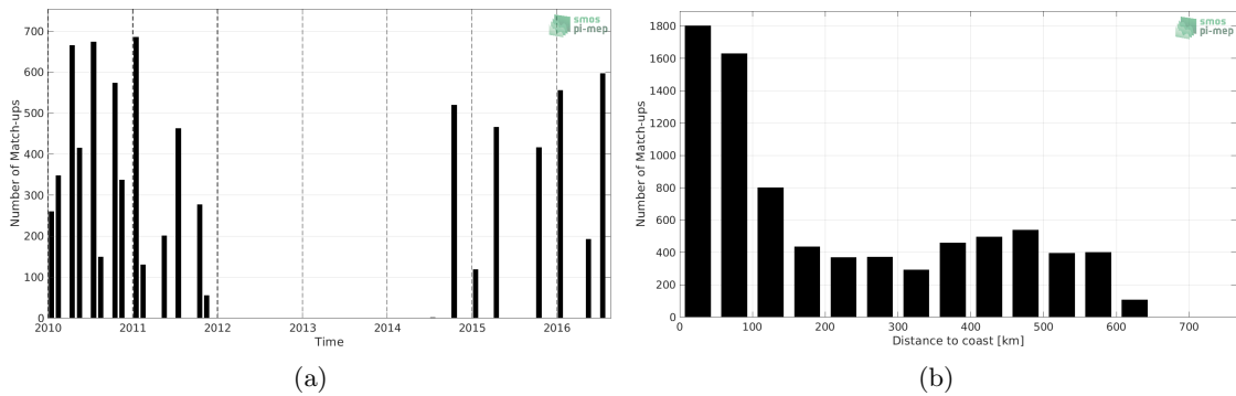
Figure 1: Number of match-ups between TSG (LEGOS-DM) and CCI SSS L4 Merged-OI v3.2 - 30-day running (ESA) SSS as a function of time (a) and as function of the distance to coast (b) over the Ganga and Brahmaputra river plumes Pi-MEP region and for the full satellite product period.
