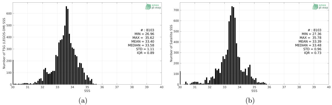
Figure 2: Histograms of SSS from TSG (LEGOS-DM) (a) and CCI SSS L4 Merged-OI v3.2 - 30-day running (ESA) (b) considering all match-up pairs per bins of 0.1 over the Ganga and Brahmaputra river plumes Pi-MEP region and for the full satellite product period.
