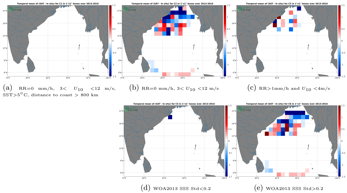
Figure 11: Temporal mean gridded over spatial boxes of size 1°x1° of \Delta SSS (CCI SSS L4 Merged-OI v3.2 - 30-day running (ESA) - Surface drifters) for 5 different subdatasets corresponding to:RR=0 mm/h, 3 < U_{10} < 12 m/s, SST>5°C, distance to coast > 800 km (a), RR=0 mm/h, 3 < U_{10} < 12 m/s (b), RR>1mm/h and U_{10} < 4 m/s (c), WOA2013 SSS Std<0.2 (d), WOA2013 SSS Std>0.2 (e).
