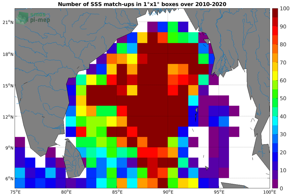
Figure 4: Number of SSS match-ups between Argo SSS and the CCI SSS L4 Merged-OI v3.2 - 30-day running (ESA) SSS product for the Ganga and Brahmaputra river plumes Pi-MEP region over 1°x1° boxes and for the full satellite product period.
