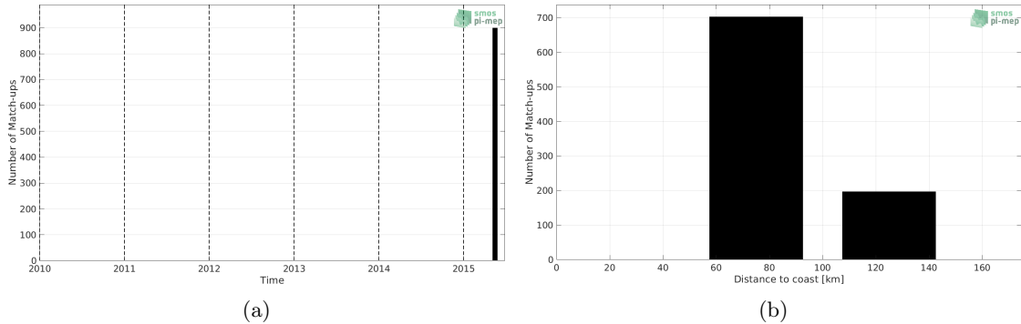
Figure 1: Number of match-ups between TSG (SAMOS) and CCI SSS L4 Merged-OI v2.31 - 30-day running (ESA) SSS as a function of time (a) and as function of the distance to coast (b) over the Ganga and Brahmaputra river plumes Pi-MEP region and for the full satellite product period.
