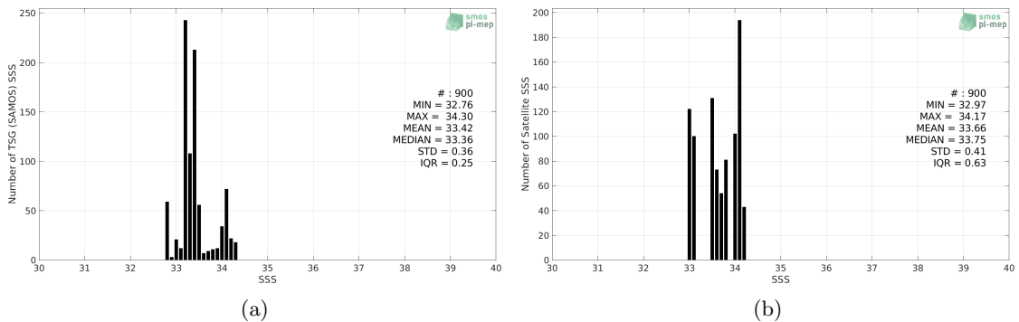
Figure 2: Histograms of SSS from TSG (SAMOS) (a) and CCI SSS L4 Merged-OI v2.31 - 30-day running (ESA) (b) considering all match-up pairs per bins of 0.1 over the Ganga and Brahmaputra river plumes Pi-MEP region and for the full satellite product period.
