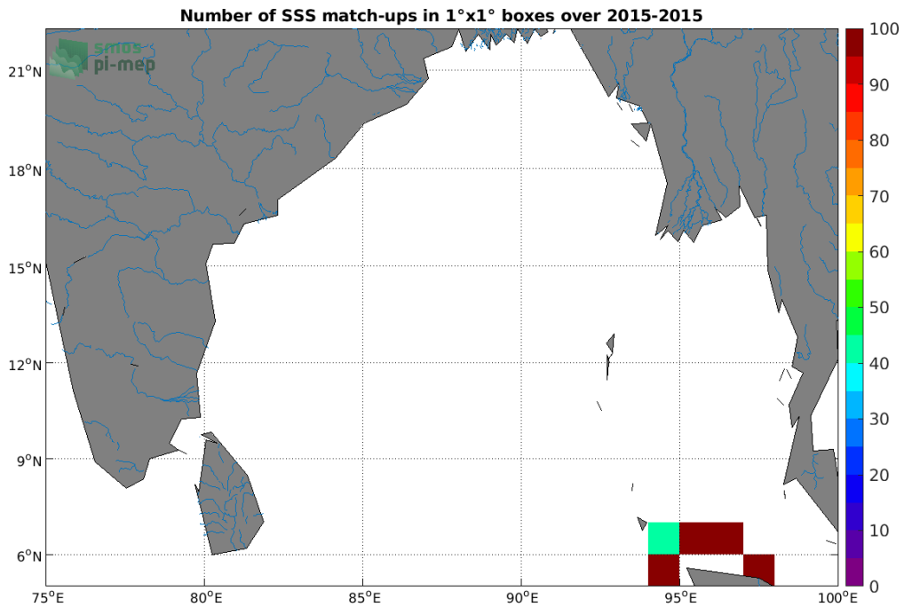
Figure 4: Number of SSS match-ups between TSG (SAMOS) SSS and the CCI SSS L4 Merged-OI v2.31 - 30-day running (ESA) SSS product for the Ganga and Brahmaputra river plumes Pi-MEP region over 1^\circ \times 1^\circ boxes and for the full satellite product period.
