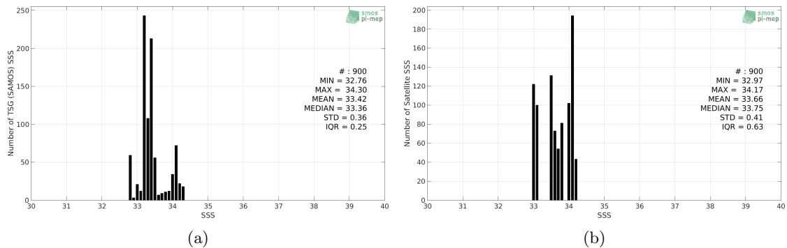
Figure 2: Histograms of SSS from TSG (SAMOS) (a) and CCI L4 Merged-OI v2.31 - 30-day running (ESA) (b) considering all match-up pairs per bins of 0.1 over the Ganga and Brahmaputra river plumes Pi-MEP region and for the full satellite product period.
