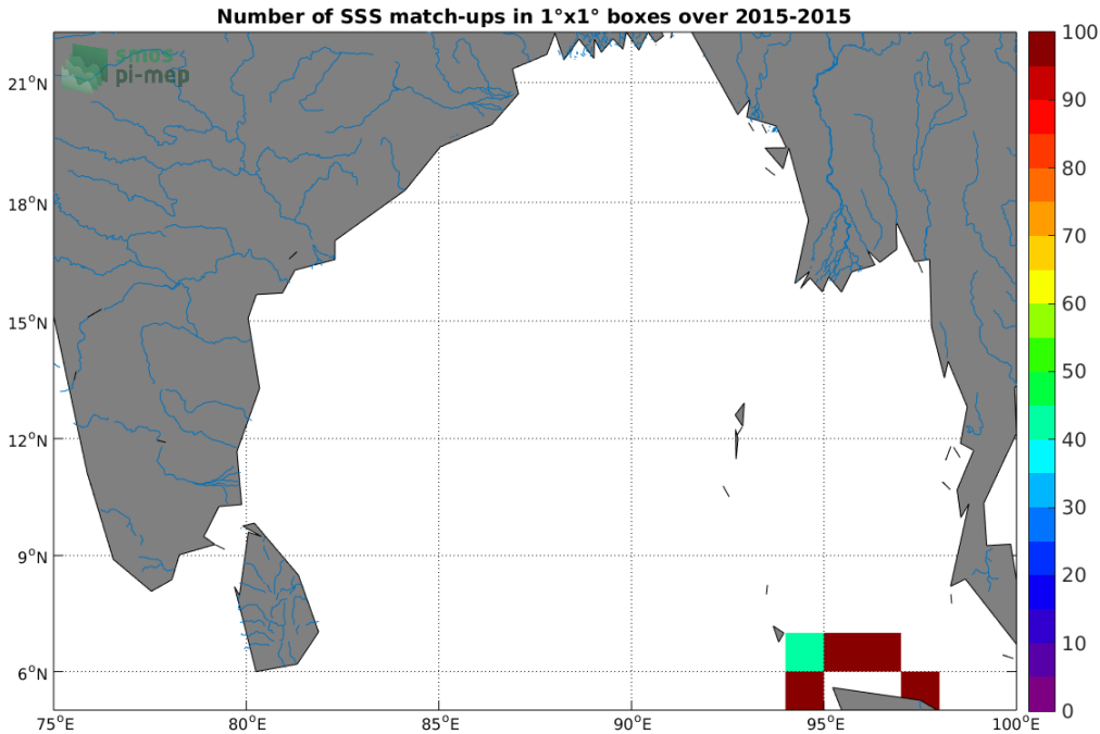
Figure 4: Number of SSS match-ups between TSG (SAMOS) SSS and the CCI L4 Merged-OI v2.31 - 30-day running (ESA) SSS product for the Ganga and Brahmaputra river plumes Pi-MEP region over 1°x1° boxes and for the full satellite product period.
